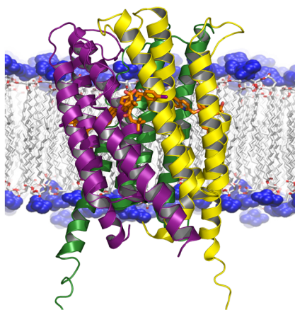
Figure 2. Crystal structure of the key enzymes and proteins in leukotriene biosynthesis. (A) Structure of 5-LOX at 2.4 Å resolution depicting the N-terminal \beta -barrel domain (yellow) and the catalytic domain (magenta). (B) Structure of FLAP at 4 Å resolution. It is a trimer with each monomer (yellow, green, and magenta) composed of four transmembrane \alpha -helices. FLAP inhibitors are bound in the intermonomeric cleft. (C) Structure of LTA4H at 1.9 Å resolution. The protein is folded into three domains, an N-terminal (yellow), a catalytic (green), and a C-terminal (magenta), between which the catalytic center is located. A molecule of LTA 4 is indicated in the center of the interdomain cavity. (D) Structure of LTC4S. It is a trimer with each monomer (yellow, green, and magenta) composed of 4 transmembrane \alpha -helices. Three molecules of the cosubstrate GSH are bound between two monomers toward the cytosolic side of the protein. Figures were derived from the following Protein Data Bank IDs: 5-LOX 3O8Y; FLAP 2Q7R; LTA4H 5NI6; LTC4S 2UUH.
