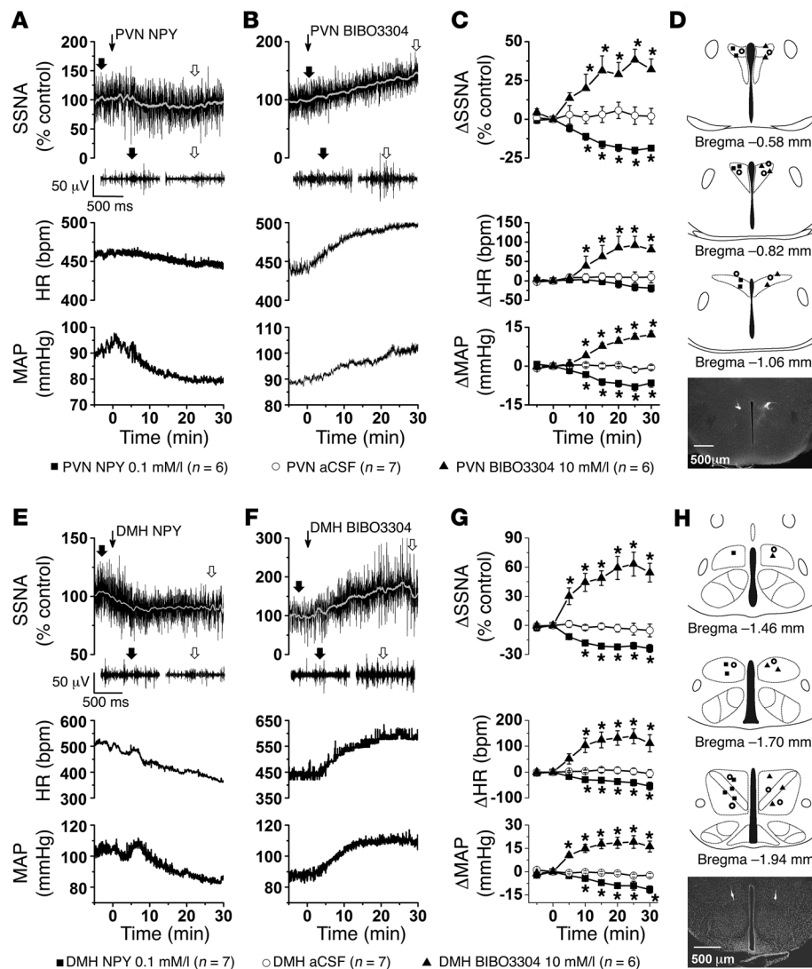
Figure 3. Bilateral nano-injections of NPY or BIBO3304 into the PVN and DMH of WT mice decrease and increase SSNA, HR, and MAP, respectively. (A and E). Representative experiments showing that injections (at thin arrow) of NPY into the PVN or DMH decrease raw SSNA, HR, and MAP. (B and F) Representative experiments showing that injections (at thin arrow) of BIBO3304 into the PVN or DMH increase raw SSNA, HR, and MAP. (C) Grouped data showing that PVN NPY or BIBO3304 decreases or increases SSNA, HR, and MAP, respectively; PVN injections of aCSF had no effects. Baseline values were 88 \pm 3 mmHg and 443 \pm 15 bpm ( n = 19 ). (G) Grouped data showing that DMH injections of NPY or BIBO3304 decrease or increase SSNA, HR, and MAP, respectively; DMH injections of aCSF had no effects. Baseline values were 86 \pm 2 mmHg and 450 \pm 12 bpm ( n = 20 ). (D and H) Histological maps (based on ref. 80), and representative sections illustrating PVN and DMH injection sites. *P < 0.05 , compared with time 0.
