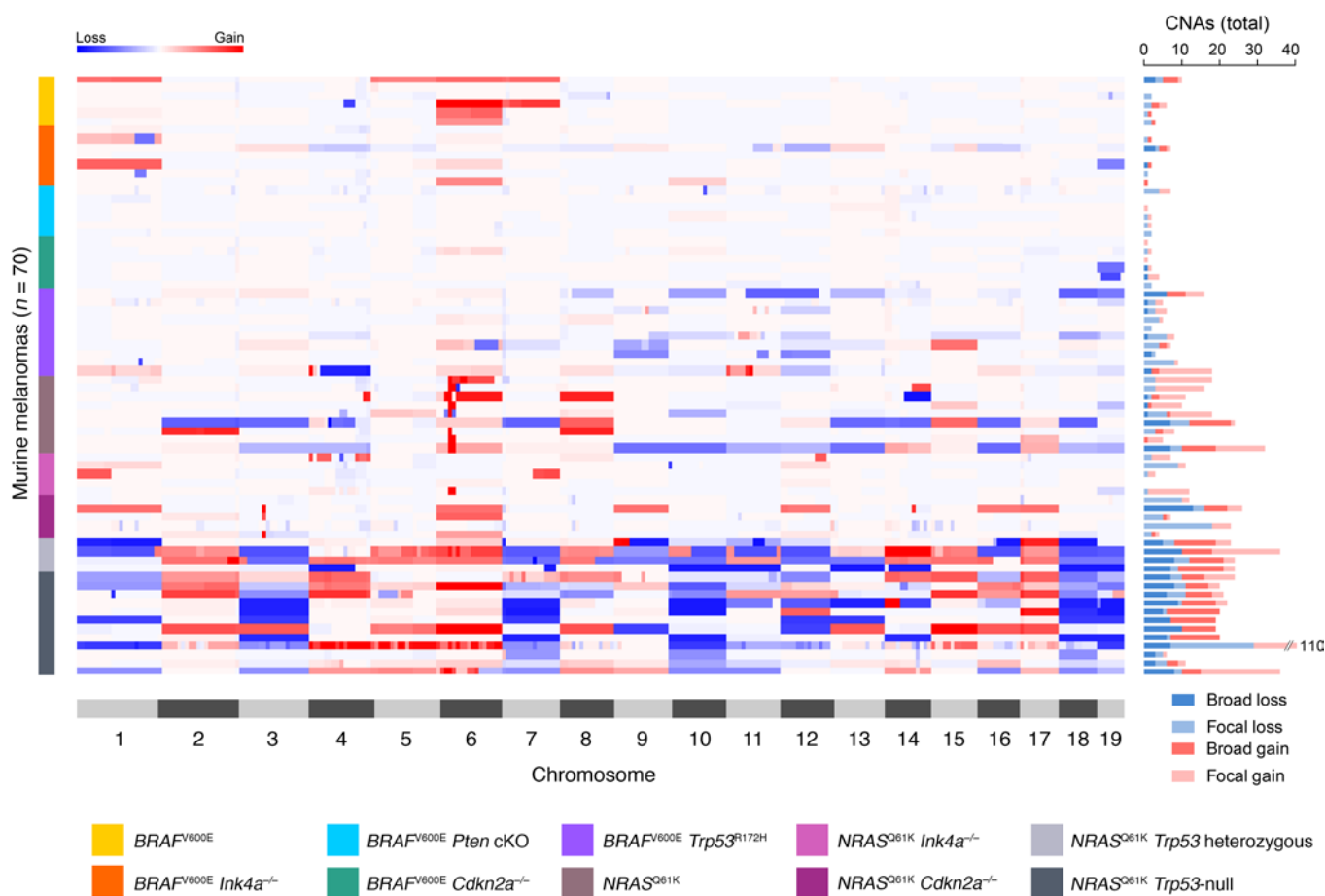
Figure 1. Landscape of CNAs in genetically induced murine melanomas. Heat map of CNAs in 70 BRAF^{V600E} - and NRAS^{Q61K} -driven murine melanomas. The genetic background of each sample is color coded based on the legend provided at the bottom of the panel. The copy-number gains and losses are depicted in red and blue, respectively. Chromosome numbers are shown on the x axis. The total number of CNAs (focal and broad) is shown on the right panel.
