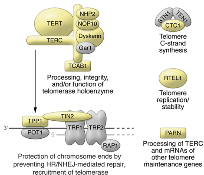
Figure 3. Schematic representation of human proteins affected by germline mutations in dyskeratosis congenita and related disorders. Mutations affecting 11 different proteins have been reported to date in dyskeratosis congenita and related disorders, as indicated by colored structures. TERT, TERC, dyskerin, NHP2, NOP10, and TCAB1 are important for the processing, integrity, and/or function of the telomerase holoenzyme, a ribonucleoprotein complex containing TERC RNA and the catalytic TERT protein with reverse transcriptase activity. TIN2 and TPP1 (encoded by ACD ) are members of the shelterin complex (see Figure 1). CTC1 belongs to a complex that regulates telomere C-strand synthesis and telomere replication. RTBL1 is important for telomere replication and stability. PARN was recently described to control processing of TERC RNA as well as mRNAs of other telomere maintenance genes.
