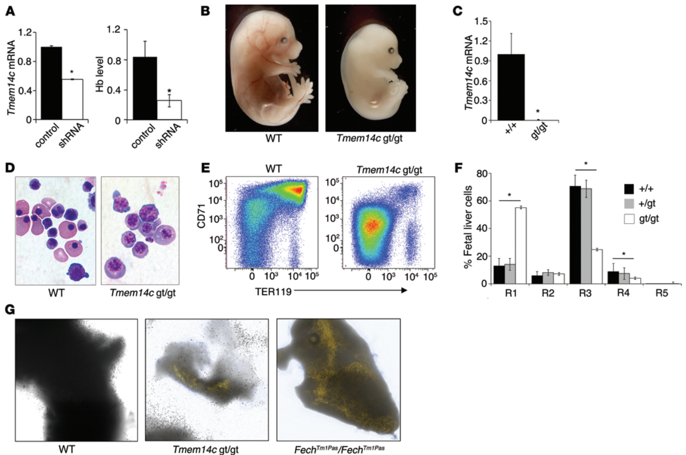
Figure 3. TMEM14C is specifically required for terminal differentiation of primary definitive murine erythroid cells. (A) Primary murine fetal liver cells transduced with shRNA lentivirus, silencing the expression of Tmem14c mRNA, have significantly decreased hemoglobinization, compared with control cells. (B) E15.5 Tmem14c gt/gt mice are profoundly anemic; their livers are deficient in hemoglobinization compared with wild-type littermates (original magnification, \times 20 ). (C) Tmem14c mRNA expression is abrogated in fetal livers derived from E12.5 Tmem14c gt/gt embryos. (D) Erythroid cells (original magnification, \times 100 ) from E12.5 Tmem14c gt/gt embryos are developmentally arrested. (E) Erythroid maturation arrest of E12.5 Tmem14c gt/gt fetal liver population was confirmed by flow cytometry analysis of CD71 and TER119 expression. (F) Quantification of the R1–R5 subpopulations. Tmem14c gt/gt fetal liver erythropoiesis is similar to that in wild-type fetal livers. (G) Autofluorescent erythrocytes are visualized in Tmem14c gt/gt and Fech Tm1Pas / Fech Tm1Pas fetal livers under fluorescent light (original magnification, \times 630 ) ( \lambda , 405 nm excitation and \lambda , 620 nm emission; Supplemental Methods). Autofluorescent erythrocytes are not present in wild-type fetal livers. * P < 0.05 .
