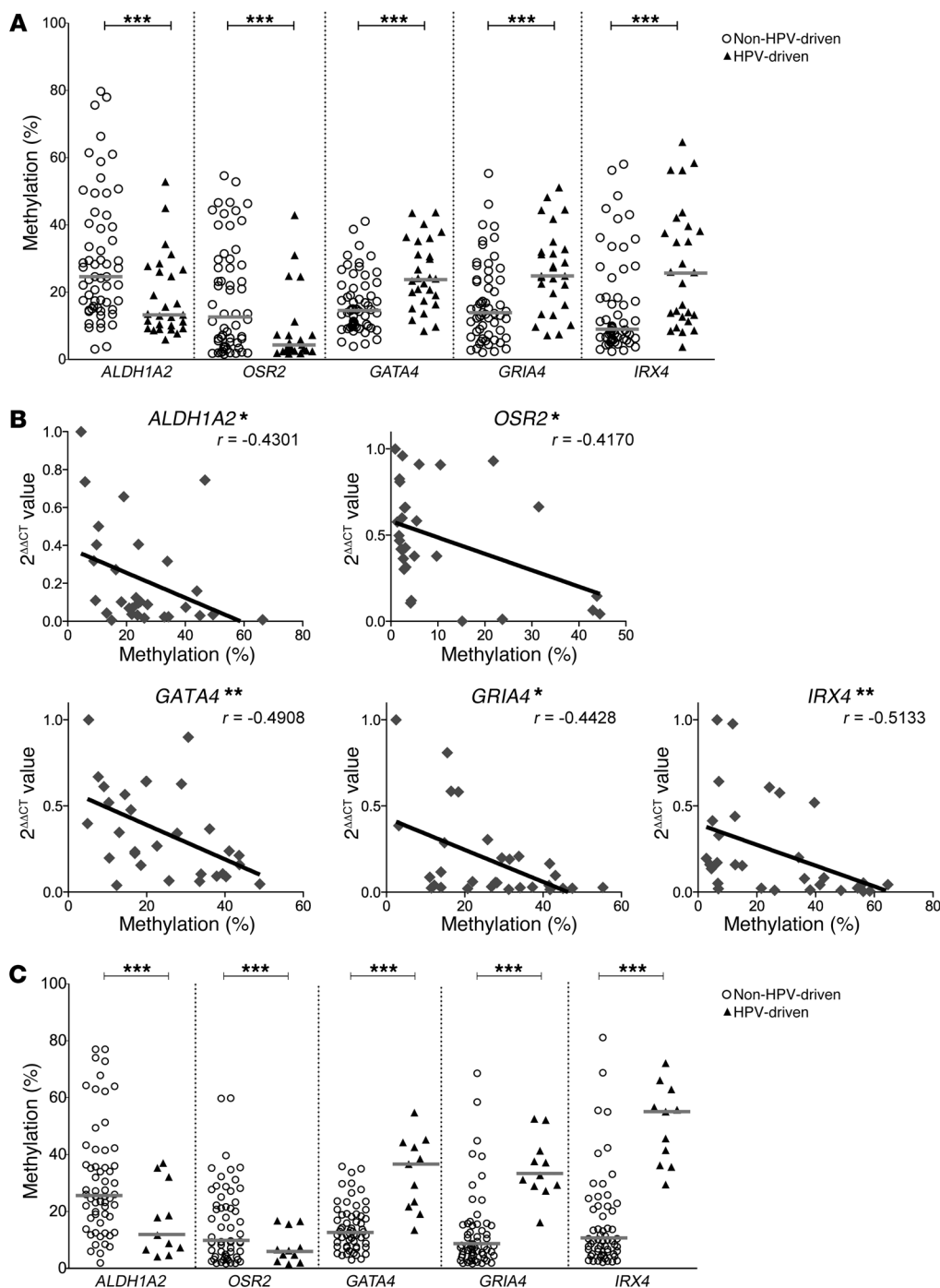
Figure 4 DNA methylation levels of gene promoter DMRs and transcript levels of ALDH1A2 , OSR2 , GATA4 , GRIA4 , and IRX4 . ( A ) Confirmation of HPV-related gene promoter methylation for ALDH1A2 , OSR2 , GATA4 , GRIA4 , and IRX4 in the combined cohort 1/2 (Heidelberg) ( n = 100 ) by MassARRAY. Each symbol represents the mean of all CpG units in a sample amplicon. Bars denote medians. *** P < 0.001 , Mann-Whitney U test. ( B ) Correlation between gene promoter methylation (mean of all CpG units) and transcript levels of 30 samples from cohort 2. Statistical nonparametric comparison for correlation between methylation and expression values was performed by Spearman's Rho method ( r is indicated). * P < 0.05 , ** P < 0.01 , 2-tailed Spearman's Rho test. ( C ) Confirmation of the discriminating methylation signature of 5 gene promoters in validation cohort 3 (Leipzig) ( n = 70 ). Each symbol represents the mean of all CpG units in a sample amplicon; bars denote medians. *** P < 0.001 , Mann-Whitney U test.
