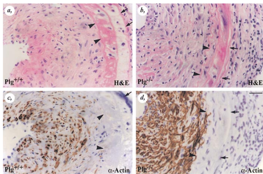
Figure 7. Light microscopic analysis of transverse sections through \text{Plg}^{+/+} (a and c) and \text{Plg}^{-/-} (b and d) carotid grafts transplanted into wild-type recipients, 45 d after transplantation. \text{Plg}^{+/+} as well as \text{Plg}^{-/-} allografts developed a large neointima within 45 d of transplantation (a and b), with all typical characteristics of adventitial remodeling, elastic lamina degradation, leukocyte infiltration into the media, medial cell proliferation, accumulation of \alpha -smooth muscle cells in the intima (c and d), and lack of fibrin-rich thrombi as observed in wild-type carotid arteries grafted into \text{Plg}^{+/+} mice. The arrowheads indicate the internal elastic laminae and the arrows the external elastic laminae. Magnification bar is 25 \mu\text{m} in all panels.
