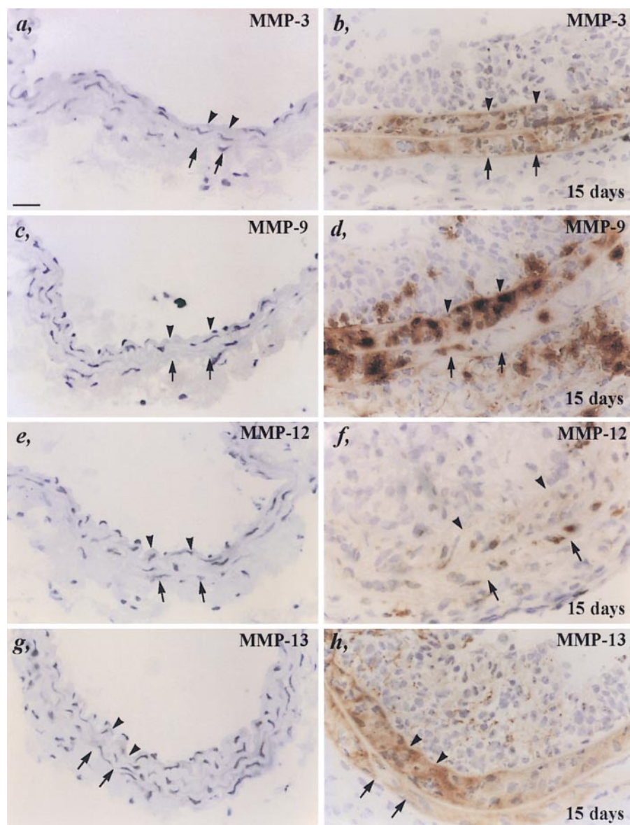
Figure 6. Immunohistochemical staining of MMP-3 (a and b), MMP-9 (c and d), MMP-12 (e and f), and MMP-13 (g and h) in transverse sections of control carotid arteries and arteries transplanted into Plg^{+/+} mice. Expression of MMPs was undetectable in normal carotid arteries (a, c, e, and g), but significantly induced in the transplanted vessels at 15 d (b, d, f, and h). MMP expression was detected for MMP-3 in the proliferating media, for MMP-9 in all three cell layers of the transplants, for MMP-12 in the medial and adventitial layers, and for MMP-13 in the proliferating media and intima. The arrowheads indicate the internal elastic laminae and the arrows the external elastic laminae. Magnification bar is 25 \mu m in all panels.
