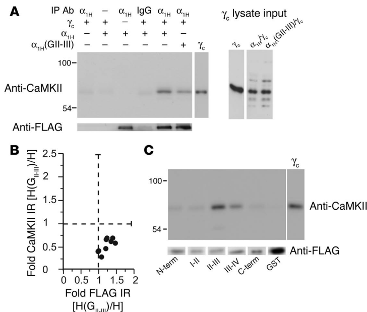
Figure 2 CaMKII \gamma_c forms a signaling complex with \alpha_{1H} channels dependent on the II-III loop. (A) Immunoblot of channel immunoprecipitates from HEK 293 cells transiently expressing FLAG-tagged \alpha_{1H} wild-type or \alpha_{1H}(GII-III) chimeric channels, most cotransfected with CaMKII \gamma_c , using: goat IgG or anti- \alpha_{1H} for the immunoprecipitation, anti-FLAG for verification of channel immunoprecipitation, and anti-CaMKII for detection of CaMKII coassociation. Input lysates show expression level of CaMKII \gamma_c with 0.25 pmol purified CaMKII \gamma_c standard for comparison. (B) An analysis of 9 experiments. Integrated optical band densities of FLAG and CaMKII immunoreactivities (IR) in \alpha_{1H}(GII-III) channel immunoprecipitates expressed relative to immunoreactivities in wild type. (C) In vitro binding of purified CaMKII \gamma_c (5 pmol/250 \mu l) to bead-bound channel intracellular domain-GST fusion proteins (2 pmol) of channel intracellular domains: N-terminus (N-term), I-II loop, II-III loop, III-IV loop, C-terminus. Shown are immunoblots of bound kinase detected by anti-CaMKII, with 0.5 pmol standard for comparison. Below is a GST blot for each fusion protein indicating nearly equal loading.
