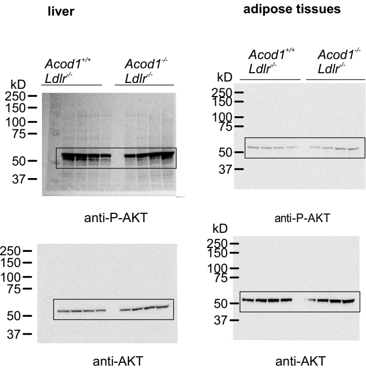
Full unedited blot/gel for Figure S3 F
