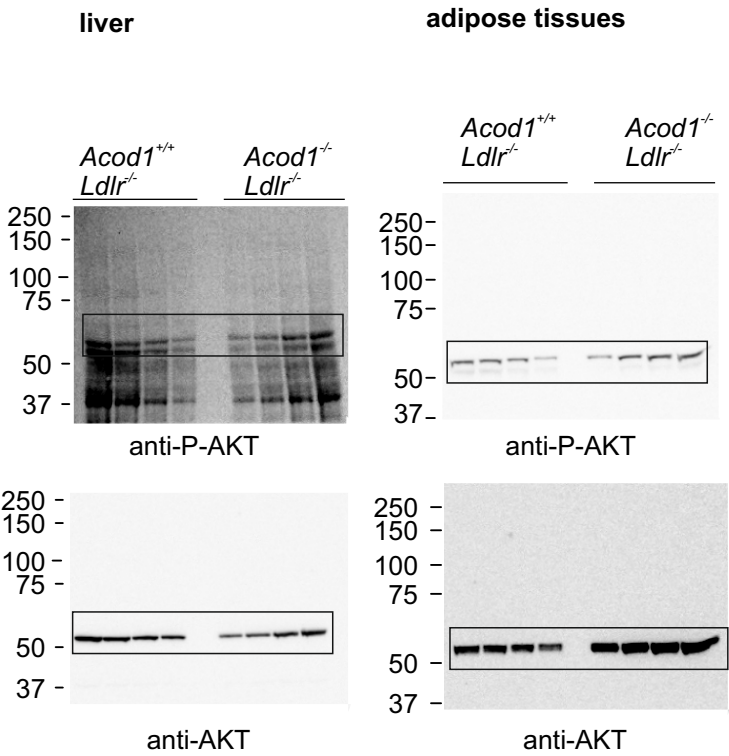
Full unedited blot/gel for Figure S3 D
