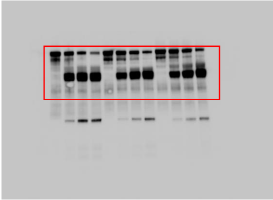
Figure 5C (Anti-Spike S2)
