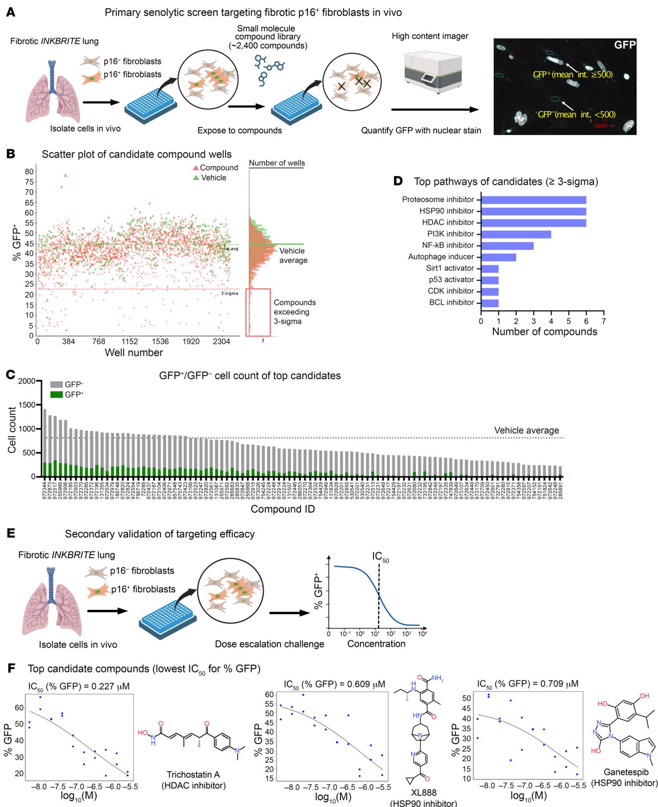
Figure 3. HTS targeting p16 ink4a fibroblasts isolated from fibrotic INKBRITE lungs. (A) Schematic outline of the HTS to identify compounds targeting p16 ink4a (GFP + ) fibroblasts from the fibrotic INKBRITE lungs. (B) Scatter plot showing hit results from each well containing compound (pink) or vehicle (green). Y-axis indicates %GFP + cells in each well after compound exposure. Compounds exceeding 3 σ for lowest %GFP were selected for validation. (C) Cell count GFP + and GFP - fibroblasts of the top senolytic candidates. (D) Biologic pathways targeted by the top senolytic candidates. (E) Schematic outline of dose-response analysis of the top senolytic candidate from the primary screen. (F) Top candidates emerging from the secondary validation using dose-response with lowest IC 50 values, including trichostatin A, XL888, and ganetespib.
