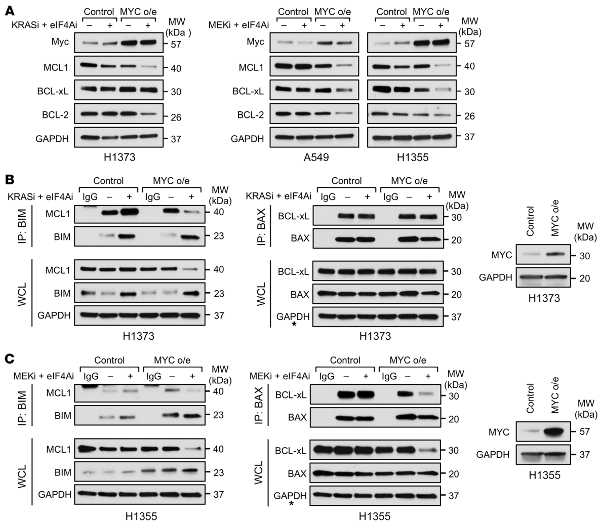
Figure 9. MYC overexpression creates a dependency on eIF4A for the expression of prosurvival proteins. (A) Immunoblots showing MCL1, BCL-xL, and BCL-2 protein levels in response to 24 hours of specified treatments in control and MYC-overexpressing resistant lines. (B and C) Immunoblots showing interactions of MCL1 and BCL-xL with immunoprecipitated proapoptotic BIM and BAX proteins, respectively, in response to specified drug treatments in control and MYC-overexpressing resistant lines. The GAPDH immunoblots denoted by asterisks, which serve as a loading control, have been duplicated from the left side of that panel, because immunoblots were all generated from the same gel and membrane. (Right) Immunoblots confirm ectopic expression of MYC by cDNAs.
