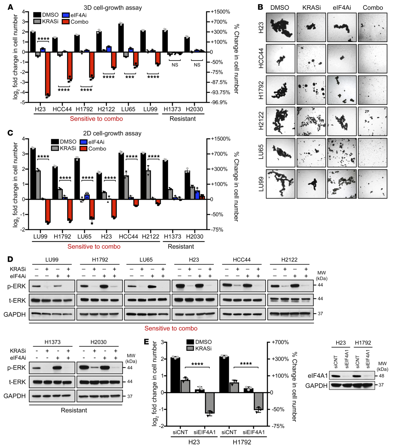
Figure 1. eIF4A inhibitors dramatically sensitize NSCLCs to KRAS G12C inhibitors. (A) Bar graph depicting the fold change in cell numbers after 72 hours (versus day 0) using a panel of KRAS G12C -mutant NSCLC cells grown in 3D conditions. Cells were treated with vehicle (DMSO), 25 nM eFT226 (eIF4Ai), 100 nM MRTX849 (KRASi), or both agents together (Combo). Data are represented as mean \pm SD. n = 3 . ***P < 0.001 ; ****P < 0.0001 , 1-way ANOVA and Tukey's post hoc test. (B) Representative photographs of sensitive KRAS G12C -mutant NSCLC spheroids after 72 hours of indicated drug treatments. Images were obtained using the 2X Bright Field channel. Original magnification, \times 2 . (C) Bar graph depicting fold change in cell numbers after 72 hours (versus day 0) in the same panel of cell lines grown in 2D tissue-culture conditions with 2% serum. Cells were treated with vehicle (DMSO), 25 nM eFT226 (eIF4Ai), 100 nM MRTX849 (KRASi), or both agents together (Combo). Data are represented as means \pm SD. n = 3 . ****P < 0.0001 , 1-way ANOVA and Tukey's post hoc test). (D) Immunoblots showing suppression of phospho-ERK by MRTX849 (KRASi, 100 nM) and/or eFT226 (eIF4Ai, 25 nM) after 24 hours of treatment. (E) Bar graphs depicting fold change in cell number of specified cell lines transfected with either siCNT or siEIF4A1 and treated with vehicle (DMSO) or 100 nM MRTX849 (KRASi) for 72 hours in 2D/low-serum conditions. Data are represented as means \pm SD. n = 3 . ****P < 0.0001 , 1-way ANOVA and Tukey's post hoc test. Immunoblots confirm suppression of eIF4A1 by siRNAs.
