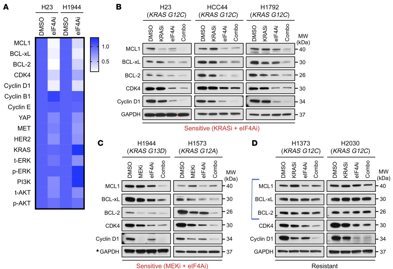
Figure 5. eIF4A and RAS pathway inhibitors cooperatively suppress the expression of prosurvival BCL-2 family proteins, cyclin D1, and CDK4. (A) Heatmap depicting protein expression of established eIF4A-regulated targets in H23- and H1944-sensitive lines after 24 hours of treatment with vehicle (DMSO) or eFT226 (eIF4Ai). Protein expression was normalized by GAPDH. Raw data from Western blots are shown in Supplemental Figure 3. (B and C) Immunoblots of MCL1, BCL-xL, BCL-2, CDK4, and cyclin D1 protein levels in sensitive cell lines after 24 hours of specified treatments. *For H1944, the loading control is the same as shown in Figure 2B because protein expression was tested using the same membrane. (D) Immunoblots of the same targets in resistant cell lines after 24 hours of specified treatments.
