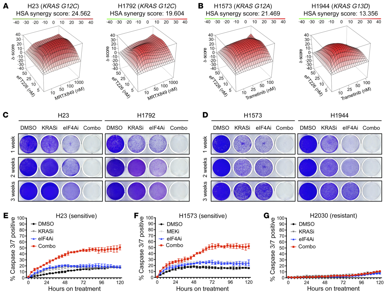
Figure 3. eIF4A inhibitors synergize with KRAS G12C or MEK inhibitors and trigger apoptosis in NSCLCs. (A and B) Synergy plots depicting the effects of indicated drug combinations using the HSA model. (C and D) Long-term cell proliferation assay of KRAS -mutant NSCLC cells treated with vehicle (DMSO), 25 nM eFT226 (eIF4Ai), 100 nM MRTX849 (KRASi), 50 nM trametinib (MEKi), or drug combinations (Combo) up to 3 weeks. (E–G) Incucyte live-cell imaging data depicting cleaved caspase-3/7 activity in sensitive H23 and H1573 and resistant H2030 cell lines in response to vehicle (DMSO), 25 nM eFT226 (eIF4Ai), 100 nM MRTX849 (KRASi), 50 nM trametinib (MEKi), or drug combinations (Combo).
