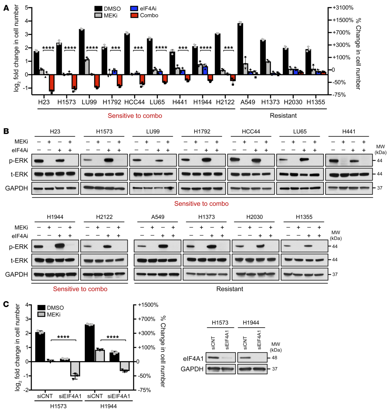
Figure 2. eIF4A inhibitors similarly enhance the effects of MEK inhibitors. (A) Bar graph depicting fold change in cell numbers in NSCLC cell lines harboring various mutations in KRAS treated with vehicle (DMSO), 25 nM eFT226 (eIF4Ai), 50 nM trametinib (MEKi), or both agents together (Combo) for 72 hours in 2D/low-serum conditions. Data are represented as means \pm SD. n = 3 . ***P < 0.001 ; ****P < 0.0001 , 1-way ANOVA and Tukey's post hoc test. H23 ( KRAS G12C ), H1573 ( KRAS G12A ), LU99 ( KRAS G12C ), H1792 ( KRAS G12C ), HCC44 ( KRAS G12C ), LU65 ( KRAS G12C ), H441 ( KRAS G12V ), H1944 ( KRAS G13D ), H2122 ( KRAS G12C ), A549 ( KRAS G12S ), H1373 ( KRAS G12C ), H2030 ( KRAS G12C ), H1355 ( KRAS G13C ). (B) Immunoblots for each cell line showing suppression of phospho-ERK by trametinib (MEKi) after 24 hours. (C) Bar graphs depicting fold change in cell numbers of specified cell lines transfected with either siCNT or siEIF4A1 and treated with vehicle (DMSO) or 50 nM trametinib (MEKi) for 72 hours in 2D/low-serum conditions. Data are represented as means \pm SD. n = 3 . ****P < 0.0001 , 1-way ANOVA and Tukey's post hoc test. Immunoblots confirm suppression of eIF4A1 by siRNAs.
