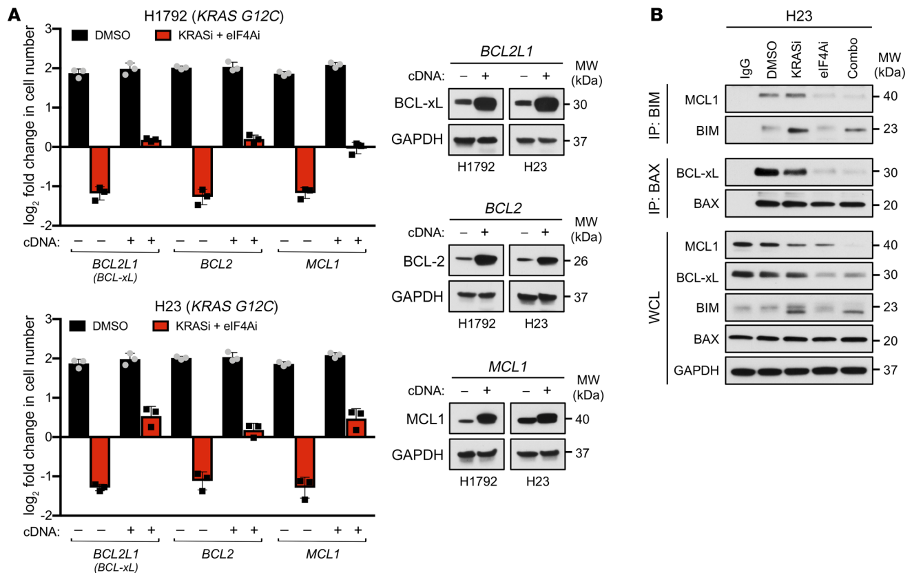
Figure 7. Reconstitution with survival proteins prevents cell death in response to eIF4A and KRAS G12C inhibitors. (A) (Left) Bar graphs depicting fold changes in cell numbers of H23 and H1792 cells ectopically expressing BCL2L1 (BCL-xL), BCL2 , or MCL1 cDNAs treated for 72 hours with combined 25 nM eFT226 (eIF4Ai) and 100 nM MRTX849 (KRASi). Data are represented as means \pm SD. n = 3 . (Right) Immunoblots confirming overexpression of BCL-xL, BCL-2, and MCL1 by cDNAs. (B) Immunoblots showing interactions of MCL1 and BCL-xL with immunoprecipitated proapoptotic BIM and BAX proteins, respectively, in response to specified drug treatments in sensitive H23 cells.
