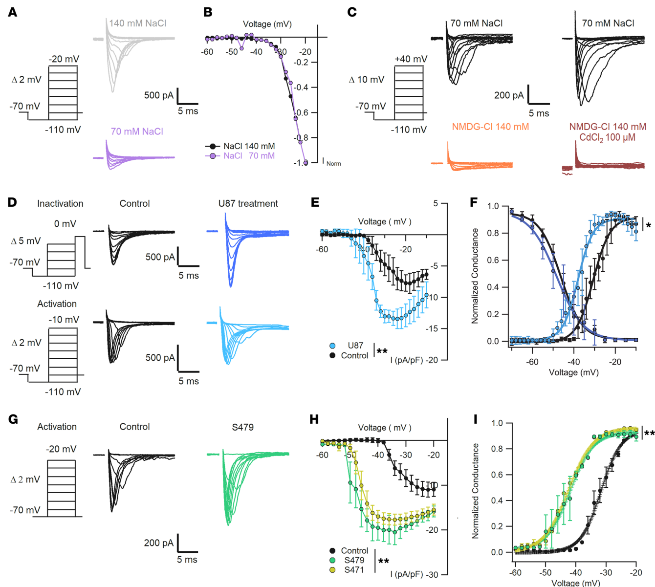
Figure 5. Increased spontaneous firing is associated with a shift of the activation curve of the inward voltage-dependent Na + current. (A) Representative traces of voltage-dependent Na + current activation in the presence of 140 mM (gray) and 70 mM (purple) NaCl. (B) Normalized currents in A show similar voltage activation dependence. Kruskal-Wallis test, P > 0.05 , n = 5 . (C) Replacement of NaCl by NMDG-Cl shows a residual small inward current (orange) blocked by addition of CdCl 2 100 \mu M (brown); n = 5 . (D) Representative traces of voltage-dependent Na + currents obtained with CdCl 2 100 \mu M in the extracellular solution and internal solution with CsCl 135 mM plus NaCl 5 mM. Currents were recorded with the protocols used for activation and inactivation in control (black; n = 7-10 ) and U87 exosome-treated (blue; n = 12-14 ) neurons. (E) I-V curve comparing current density as in D, showing increased current in treated neurons (Kruskal-Wallis test, **P < 0.01 ). (F) Dependence of normalized conductance G/G_{\max} as a function of voltage for control and treated neurons, showing an average V_{1/2} shift of -6.4 mV (values in main text; *P < 0.05 , Mann-Whitney U test). (G) Representative traces of Na + currents activated under control conditions (black; n = 7 ) and in neurons treated for 24 hours with exosomes from patient S479 (green; n = 7 ). (H) Average I-V curves of Na + currents for control and patient exosome-treated neurons, showing higher Na + current density in cells treated with patients' exosomes ( **P < 0.01 , Kruskal-Wallis test). (I) Normalized conductance curve for the conditions in H showing early activation of the Na + conductance of neurons treated with patients' exosomes ( V_{1/2} shift of -12 \pm 7.2 mV, values in main text; **P < 0.01 , Mann-Whitney U test). Voltage clamp protocols to test Na + current activation and inactivation are shown on the left of each panel.
