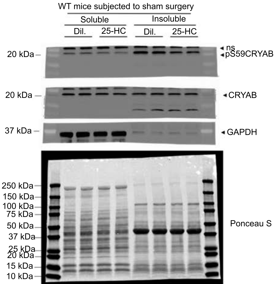
Uncropped gel western blots figure S12
