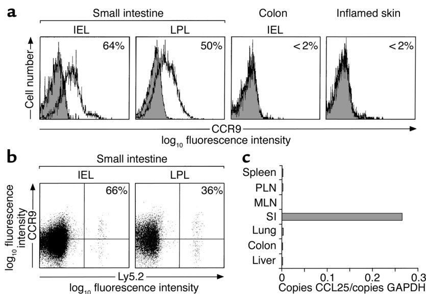
Figure 4 Activated CCR9 + OT-1 cells selectively localize to the small intestine. (a) CCR9 expression on CD8αβ + lymphocytes isolated from tissue effector sites. Cells were stained with anti-CCR9 antibody (open) or anti-CCR9 antibody that had been preincubated with the CCR9-immunizing peptide (shaded), and analyzed by flow cytometry. Results are representative stainings from six mice for small-intestinal and colonic IELs and three mice for small-intestinal LPLs. Skin CD8αβ + lymphocytes were obtained from the ears of mice with 2,4-dinitro-1-fluorobenzene-induced DTH and are from two stainings using ears pooled from a total of 40 mice. Numbers represent percentage of CD8αβ + lymphocytes that are CCR9 + with background staining removed. (b) OT-1 cells (Ly5.2 + ) were injected into C57BL/6j-Ly5.1 mice. Three days after intraperitoneal administration of OVA, lymphocytes were isolated from the small intestine, and the expression of CCR9 on OT-1 lymphocytes was determined by flow cytometry. Results are from five (IEL) and one (LPL) separate stainings using a total of eleven and three mice respectively. Numbers represent the percentage of OT-1 cells expressing CCR9 with background staining removed. (c) CCL25 is selectively expressed in the murine small intestine (SI). Quantitative analysis of CCL25 mRNA expression was determined by real-time RT-PCR.
