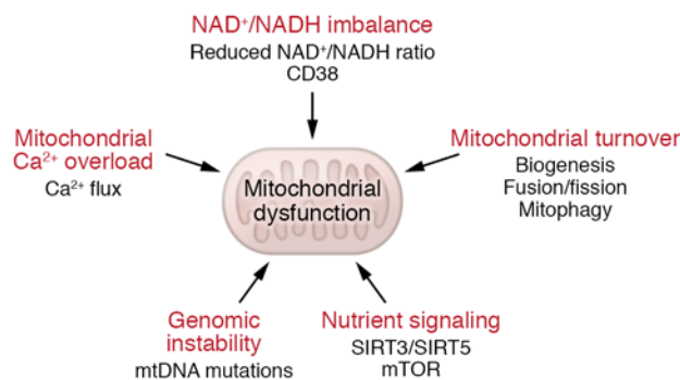
Figure 2. Mechanisms that can cause mitochondrial dysfunction. These include mtDNA mutations (genomic instability); mitochondrial turnover (as defined by the ratio of mitochondrial biogenesis and mitophagy, associated with fusion and fission); nutrient signaling through mTOR, modified by the mitochondrial sirtuins SIRT3 and SIRT5; the \text{NAD}^+/\text{NADH} ratio (which is controlled by CD38, among others); and \text{Ca}^{2+} fluxes resulting in mitochondrial \text{Ca}^{2+} overload. See text for discussion.
