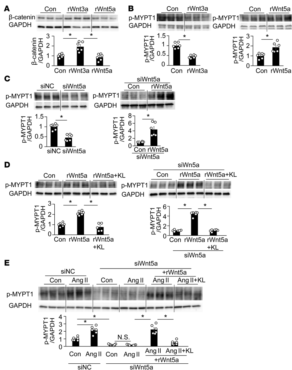
Figure 6. Wnt5a- and Ang II-induced upregulation of p-MYPT1 in cultured human VSMCs. (A) Recombinant (r) Wnt3a increased active \beta -catenin expression in cultured hVSMCs, but rWnt5a did not. n = 6 each. *P < 0.05 vs. control (Con). (B) rWnt3a decreased p-MYPT1 expression, whereas rWnt5a increased it. n = 6 each. *P < 0.05 vs. Con or rWnt5a. (C) Knockdown of Wnt5a with siRNA decreased p-MYPT1 expression relative to the negative control siRNA (siNC) (left), but the addition of rWnt5a markedly reversed it (right). n = 6 each. *P < 0.05 . (D) rKlotho (KL) inhibited rWnt5a-induced upregulation of p-MYPT1 in cells with (right) or without siWnt5a (left). n = 6 each. *P < 0.05 vs. Con or rWnt5a + KL. (E) Effects of siWnt5a on Ang II-induced increase in p-MYPT1 expression. siWnt5a significantly decreased basal (third from left) and Ang II-induced (fourth) expression of p-MYPT1, but the decrease was reversed by rWnt5a (fifth); the additional KL again inhibited p-MYPT1 expression (sixth). n = 6 each. *P < 0.05 vs. siNC-Con or siWnt5a + Ang II + Wnt5a. Data are means \pm SEM. Unpaired t tests were performed on comparisons between 2 groups. For multiple comparisons, statistical analysis was performed by Tukey-Kramer post hoc test. N.S., not significant.
