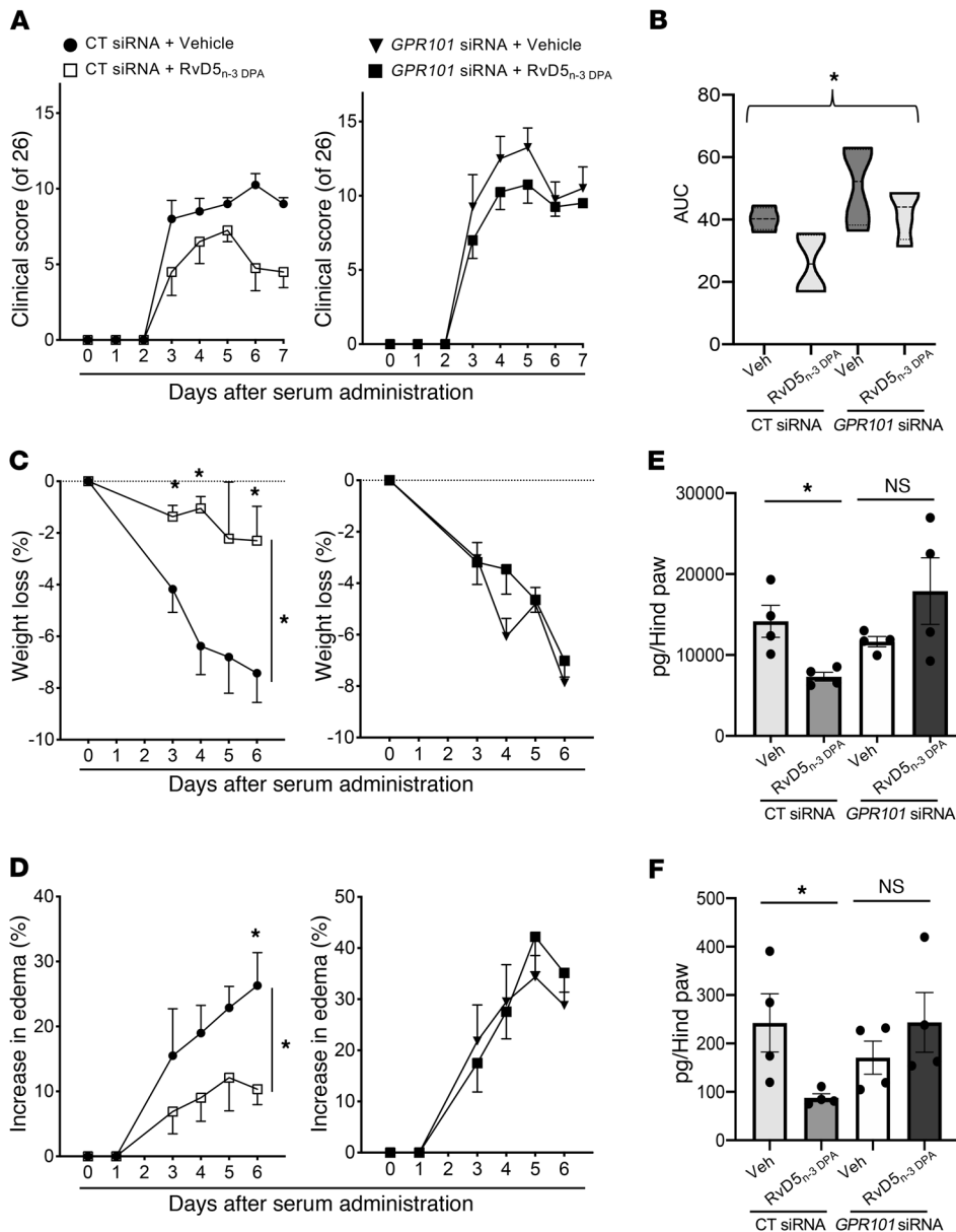
Figure 7. Knockdown of GPR101 reverses the antiarthritic actions of RvD5 n-3 DPA .
