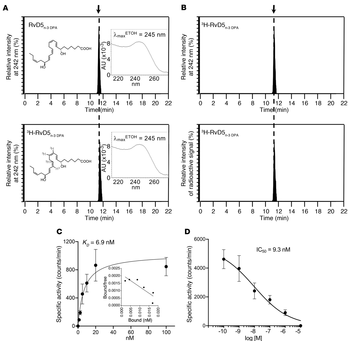
Figure 4. Specific binding of ^3\text{H} -RvD5 n-3 DPA to human GPR101. (A and B) Characterization of [10, 11, 13, 14 ^3\text{H} ]-RvD5 n-3 DPA ( ^3\text{H} -RvD5 n-3 DPA ). (A) RP-UV-HPLC chromatogram for RvD5 n-3 DPA and ^3\text{H} -RvD5 n-3 DPA . (B) RP-UV-HPLC chromatogram of ^3\text{H} -RvD5 n-3 DPA and online radioactivity monitoring. (C) GPR101-overexpressing CHO cells ( 0.5 \times 10^6 cells in 100 \mu\text{L} ) were incubated with ^3\text{H} -RvD5 n-3 DPA at the indicated concentrations in the presence or absence of 10 \mu\text{M} RvD5 n-3 DPA (60 minutes at 4°C). Cell incubations were transferred to a vacuum manifold, unbound radioligand was removed, and activity was measured. Results represent the mean \pm SEM ( n = 4 from 2 distinct experiments). Inset shows a Scatchard plot. (D) To assess competition binding, GPR101-expressing CHO cells ( 0.5 \times 10^6 cells in 100 \mu\text{L} ) were incubated with 3 nM ^3\text{H} -RvD5 n-3 DPA in the presence or absence of increasing concentrations of RvD5 n-3 DPA for 60 minutes at 4°C.
