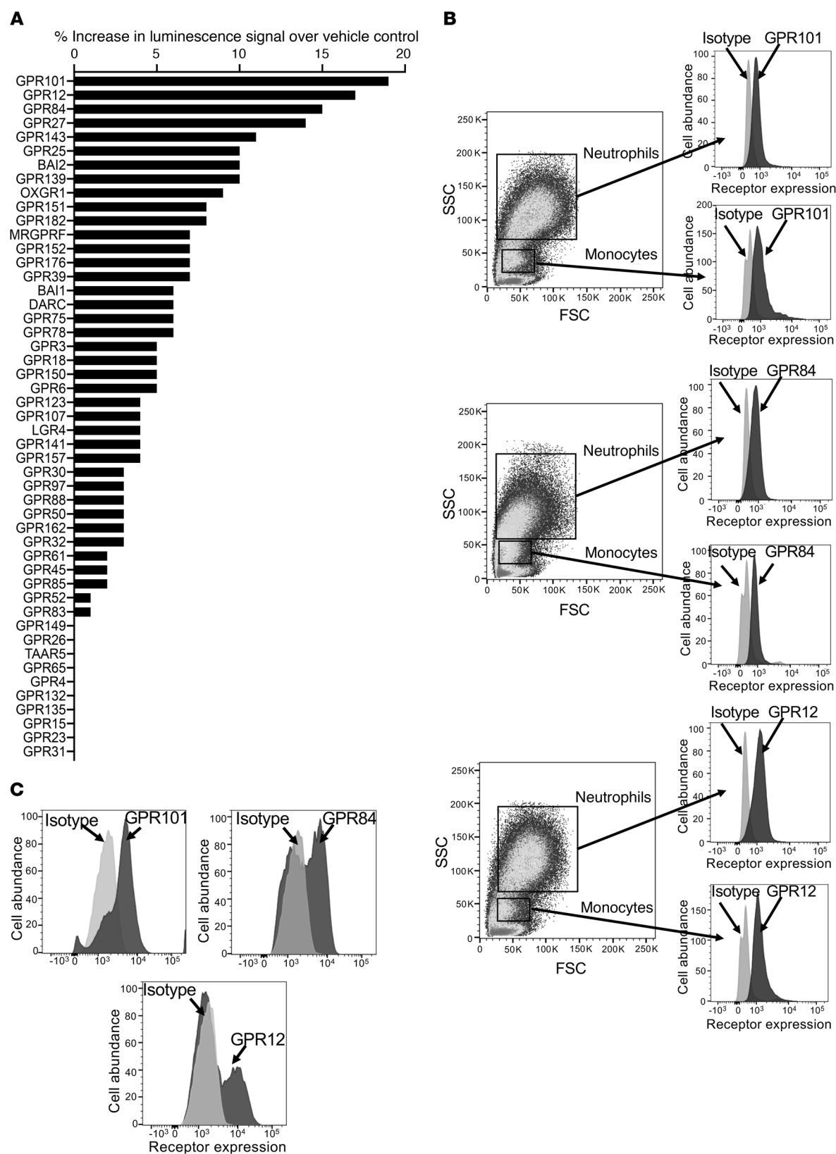
Figure 1. RvD5 n-3 DPA receptor candidates are expressed on human leukocytes. (A) Activation of orphan receptors by RvD5 n-3 DPA (10 nM). Results represent the percentage increase in luminescence signal over vehicle control. (B and C) Expression of the top 3 candidate receptors on human (B) peripheral blood leukocytes and (C) macrophages. Results are representative of 4 donors. FSC, forward scatter; SSC, side scatter.
