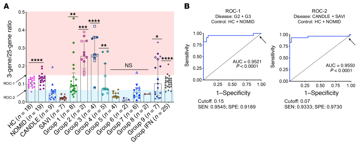
Figure 5. Ratios of 3-gene score (CXCL10 + GBP1 + SOCS1) over 25-gene score (3:25 gene ratio). (A) A ratio between 3 IFN-response genes with NF- \kappa B transcription binding sites (CXCL10, GBP1, and SOCS1) and the 25 IFN genes with no NF- \kappa B binding sites (3:25 ratio) was calculated. Depicted in the graph are the statistical significances (nonparametric Kruskal-Wallis test) from the comparisons of each group with CANDLE and SAVI patients combined: healthy controls (HC) and NOMID combined P < 0.0001 , G1 P = 0.0017 , G2 P = 0.0003 , G3 P < 0.0001 , G4 P = 0.0027 , G5 P = 0.9271 , G6 P = 0.6055 , G7 P = 0.1499 , G8 P = 0.8684 , G9 P = 0.0083 , Non-IFN P < 0.0001 . NS, not significant. Bars and error lines indicate median and interquartile range, respectively. Red shaded area indicates a high 3:25 gene ratio, blue shaded area indicates low ratio, and white area indicates normal ratio. Cutoffs were calculated in panel B. For the control groups (HC and NOMID) the same symbol is used for different individuals, as only one sample per patient is included. In all other groups, including CANDLE and SAVI, each patient is represented by a different symbol. (B) Two receiver operating characteristic (ROC) curves for the 3:25 gene ratio to distinguish HC and NOMID from patients with NDAS (G3) and LRBA deficiency (G2) (ROC-1) and CANDLE and SAVI from HC and NOMID (ROC-2) are shown. A black arrow indicates the optimal cutoff (listed under each graph). AUC, area under the curve; SEN, sensitivity; SPE, specificity. The cutoffs for the ROC curves were marked in panel A with black arrows on the y axis. A list of genes in the IFN-gene score is published in ref. 34. * P < 0.05 ; ** P < 0.01 ; *** P < 0.001 ; **** P < 0.0001 .
