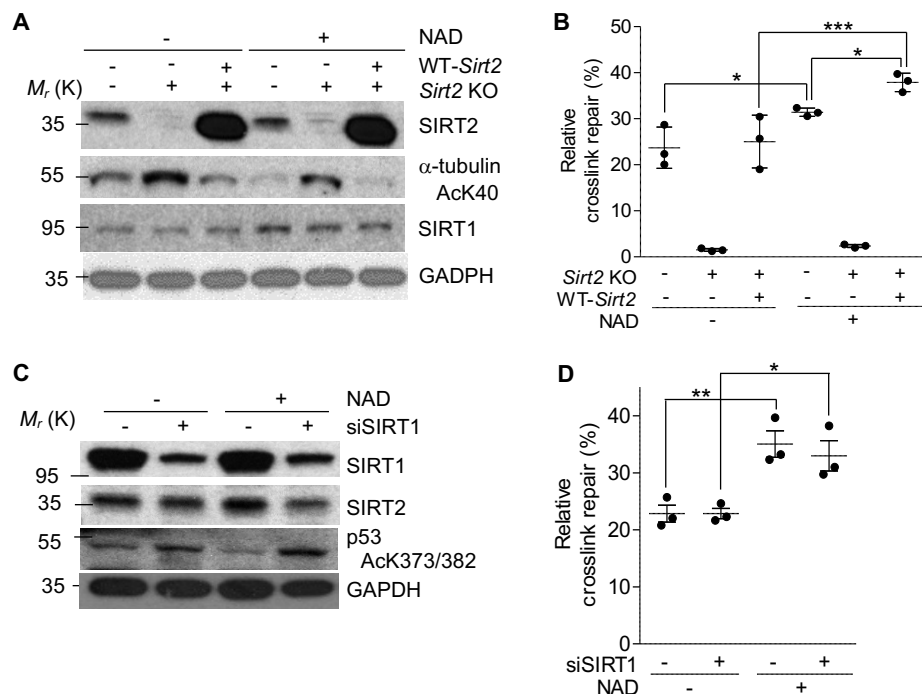
Figure 4. NAD + -mediated enhancement of NER efficiency requires SIRT2 and is independent of SIRT1.
