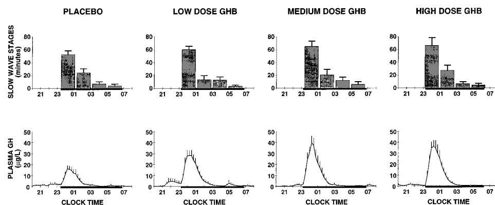
Figure 1. Mean (+ SEM) profiles of SW sleep and plasma GH in the four treatment conditions. The drug was given at 2245. The amounts of SW sleep (upper panel) are shown for successive 2-h periods from 2300 to 0700. Black bars denote the sleep periods.
