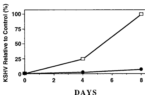
Figure 1. Time course of KSHV release from TPA-induced BCBL-1 cells in the absence (open rectangles) or presence (closed circles) of foscarnet (250 \mu M).
