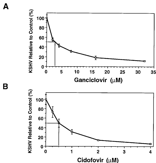
Figure 3. IC 50 determinations for ganciclovir (A) and cidofovir (B) inhibition of KSHV production. IC 50 values are indicated by the vertical lines intercepting the curves. Values are the mean, and error bars indicate the range of triplicate determinations.
