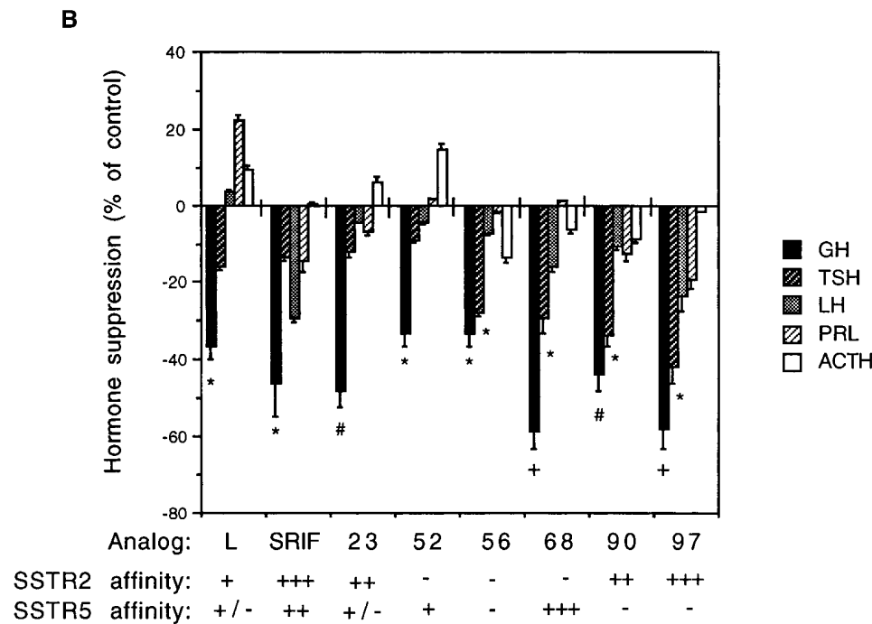
Figure 2. Human pituitary hormone suppression by SRIF analogs exhibiting different SSTR subtype specificity. Human fetal pituitaries were harvested between 23 and 25 wk gestation, cells were cultured ( 5 \times 10^4 cells/well) and 72 h later treated with different SRIF analogs (1 nM, A ; 10 nM, B ) in serum-free defined medium for 4 h. Control wells were treated with vehicle solution. Each bar represents mean ( \pm SEM) suppression of hormone secretion in four to five wells compared with control wells. L, Lanreotide ® ; SRIF, SRIF-14; 23, BIM-23023; 52, BIM-23052; 56, BIM-23056; 68, BIM-23268; 90, BIM-23190; 97, BIM-23197. * P < 0.05 ; # P < 0.005 ; + P < 0.0001 .
