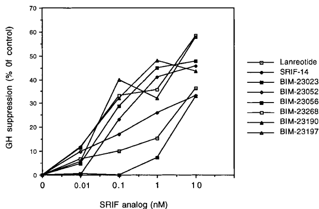
Figure 3. Human GH release from primary fetal pituitary cell cultures treated with SRIF analogs exhibiting different SSTR subtype affinities. For each indicated analog, a dose-dependent GH inhibition curve was plotted by combining the results of four experiments with the indicated doses. Maximal inhibition was achieved with 10 nM, and no further effect was seen with 100 nM. Each value represents mean suppression of GH secretion in four to five wells treated with the same analog compared with control wells in the same experiment.
