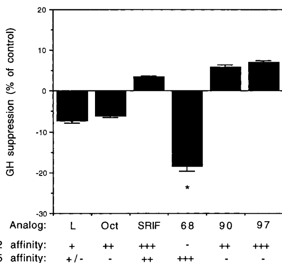
Figure 6. Human GH suppression in primary cultures derived from an invasive GH-secreting adenoma treated with SRIF analogs (10 nM) for 4 h in serum-free defined medium. L, Lanreotide ® ; Oct, Octreotide ® ; SRIF, SRIF-14; 68, BIM-23268; 90, BIM-23190; 97, BIM-23197. * P < 0.05.
