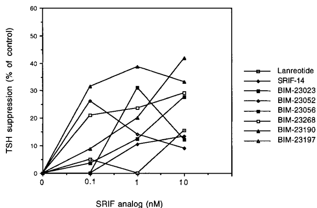
Figure 5. Dose-dependent human TSH suppression from primary fetal pituitary cultures treated with SRIF analog compounds. Each curve is a combination of three doses of the indicated compound. Each value represents mean inhibition of TSH release in four to five wells compared with control cells from the same fetal pituitary.
