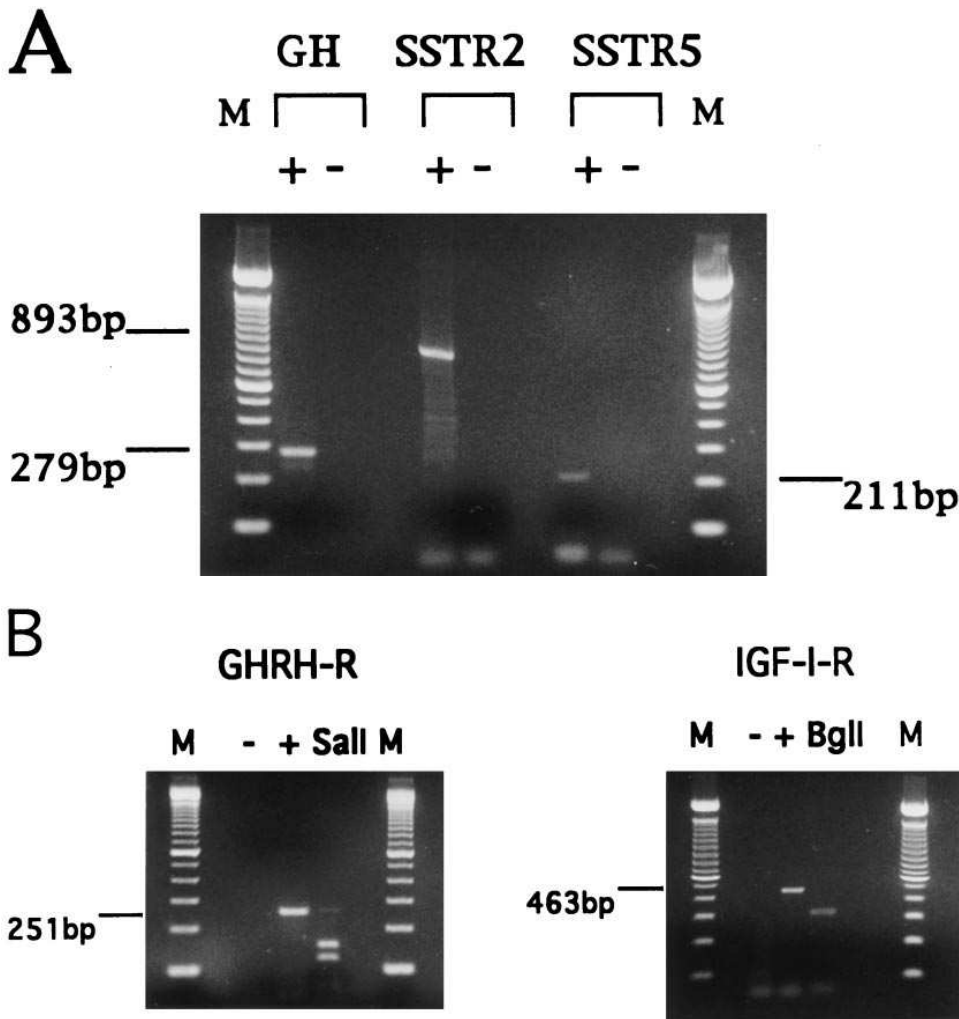
Figure 1. Somatostatin receptors (A), GHRH receptor ( GHRH-R ), and IGF-I receptor ( IGF-I-R ) mRNA expression (B) in 25-wk gestation human fetal pituitary. Extracted RNA (1 \mu g/reaction) was treated with deoxyribonuclease and subjected to reverse transcription using Oligo(dT) as primer. Samples incubated without RT enzyme served as controls. Aliquots from the generated cDNAs and the negative controls were subjected to subsequent PCR amplification (40 cycles) of GH, SSTR2, SSTR5, GHRH, and IGF-I receptors, using the primer pairs indicated in Methods. PCR products and enzyme digestion products were resolved on a 1.5% agarose gel. The expected PCR products of GH (279 bp), SSTR2 (893 bp), and SSTR5 (211 bp) are depicted in A (lane M, 100-bp DNA ladder; +, with RT; -, no RT added), and GHRH receptor (251-bp band, digested by Sal I), and IGF-I receptor (463-bp band, digested by Bgl I) are shown in B.
