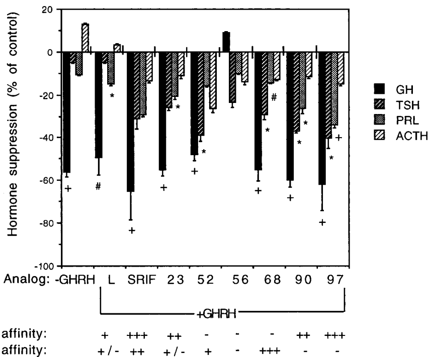
Figure 4. Human fetal pituitary hormone suppression in primary cell cultures cotreated with different SRIF analogs (10 nM) and human GHRH (1-29)NH 2 (10 nM) in serum free defined medium for 4 h. Control wells were treated with GHRH only. Each bar represents mean \pm SEM suppression of hormone secretion in four to five wells compared with control wells. -GHRH represents cells incubated without SRIF analogs or GHRH (vehicle only). L, Lanreotide ® ; SRIF, SRIF-14; 23, BIM-23023; 52, BIM-23052; 56, BIM-23056; 68, BIM-23268; 90, BIM-23190; 97, BIM-23197. * P < 0.05 ; # P < 0.005 ; + P < 0.0001 .
