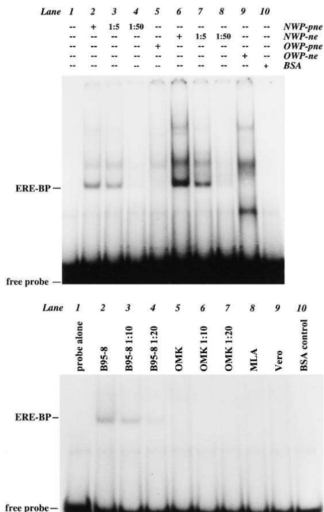
Figure 1. Specificity of the NWP ERE-BP for the ERE. The top shows that both postnuclear ( NWP-pne , lanes 2–4) as well as nuclear extracts ( NWP-ne , lanes 6–8) of the steroid-resistant B95-8 cell line contain an ERE-BP that binds to a consensus ERE. Serial dilution of the postnuclear and nuclear extracts results in disappearance of the ERE-BP-ERE complex (lanes 3 and 4, and 7 and 8, respectively). The labeled ERE-BP-ERE complex was not identified when extracts of a similarly prepared OWP B cell line were used in EMSA (lanes 5 and 9). Control lanes containing probe alone (lane 1) and BSA (lane 10) matched for protein concentration with the cell extracts used demonstrate no specifically retarded bands. The bottom shows the specificity of ERE-BP-ERE complex formation for serially diluted extract obtained from NWP cells with the steroid-resistant phenotype in vivo (lanes 2–4). ERE-BP-ERE complex was noted only in the B-lymphoblastoid cell line B95-8 but not in renal epithelial cell lines from the owl monkey ( OMK ) and green monkey ( Vero ) or in B-lymphoblasts from a gibbon ( MLA ).
