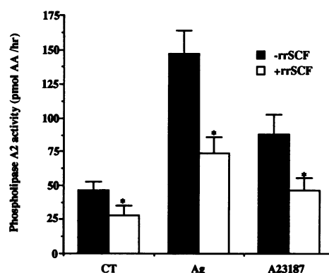
Figure 2. Effect of rrSCF on the secretion of PLA 2 activity by stimulated BMMCs. BMMCs that had been incubated without (−rrSCF) or with 100 ng/ml rrSCF for 24 h were stimulated with antigen or A23187 for 5 min or incubated in buffer alone (CT). Supernatant fluids were obtained by centrifugation, and PLA 2 activity was determined as described in Methods. PLA 2 activity (fatty acid release from labeled E. coli membranes) is expressed in pmol AA release/h, and these data are the means±SEM of four separate experiments performed in duplicate. * P < 0.05 ; n = 4 , ±rrSCF.
