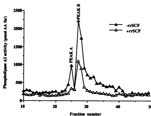
Figure 3. Partial purification of sPLA 2 from BMMCs. BMMCs that had been incubated without (−rrSCF) or with 100 ng/ml rrSCF (+rrSCF) were incubated with 0.18 M H 2 SO 4 overnight at 4°C. Extracts were neutralized, suspended in solvent A (0.1% TFA), and then loaded onto a Supercosil DP column (0.46-cm internal diameter, 24 cm long). PLA 2 activity (fatty acid release from labeled E. coli membrane) was determined in each 1-min fraction as described in Methods. PLA 2 activity is expressed as the amount of AA hydrolyzed from E. coli phospholipids (pmol/h). These data are representative of four separate experiments.
