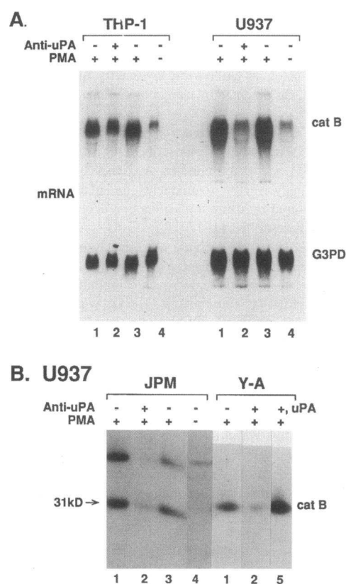
Figure 2. uPAR occupancy influences cat B mRNA expression during macrophage differentiation. (A) Whole cell RNA isolated from myeloid cells was analyzed for expression of cat B and G3PD as described. PMA-induced differentiation was either in the absence (THP-1) or presence (U937) of vit D 3 . Stimulus was either in the absence (lane 1) or presence of 175 \mu g/ml anti-uPA (lane 2), of 175 \mu g/ml rabbit nonimmune serum (lane 3); unstimulated cells were used as control (lane 4). (B) The effect of these treatments on cat B protein was assessed by labeling U937 cells obtained from a parallel plate with [ ^{125} I]JPM. Also shown by [ ^{125} I]Y-A labeling of cells obtained from a separate experiment is that 100 nM DFP-uPA (lane 5) overcomes the inhibitory effect of 125 \mu g/ml anti-uPA (lane 2). Densitometric analysis indicated that anti-uPA inhibited cat B mRNA by >50% and protein by >80%. Representative results from at least three separate experiments are shown.
