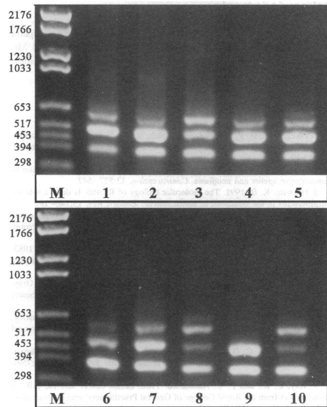
Figure 6. Size separation by electrophoresis on 1.5% agarose of RT-PCR products obtained from 1 \mu g total RNA of normal canine mammary tissue using porcine specific GH primers and human specific \beta -actin primers. After electrophoresis the gel was stained with ethidium bromide and photographed under ultraviolet illumination. The lower 383-bp band corresponds to \beta -actin. The band at 495 bp is obtained from GH mRNA while a 600-bp fragment is amplified of unknown origin. Normal mammary tissues were analyzed of dogs treated with progestins ( top ) or mammary tissue from control dogs ( bottom ). Sample 9 corresponds to the tissue sample with code P221L5 (Table I), which is normal mammary tissue of a dog treated with proligestone 1 wk before surgical removal of a malignant mammary carcinoma.
