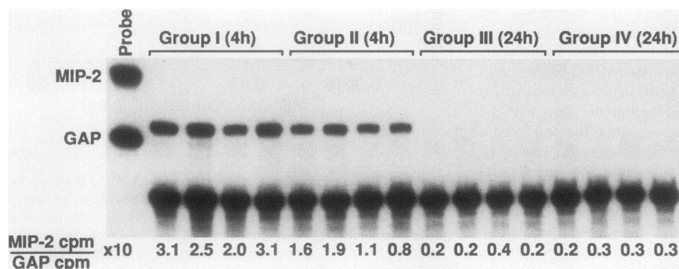
Figure 5. Expression of MIP-2 mRNA analyzed by RNase protection assay. 5 \mu g of total RNA was hybridized with riboprobes, as described in Methods. The [ \alpha^{32} P]UTP-labeled MIP-2 and GAP riboprobes were protected with the complementary mRNA from glomeruli. The gel was scanned on AMBIS, and the final values were factored relative to the GAPDH mRNA levels. In the RNase protection assay, the protected band is shorter than the probe since the polylinker regions present in the probe are not protected. Groups I and III received NRS; groups II and IV received anti-MIP-2 Ab.
