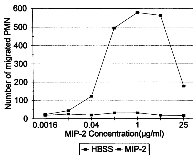
Figure 3. The in vitro chemotactic activity of the rMIP-2 is shown for one study which is representative of three done. The data are presented as the mean of triplicate wells for the numbers of PMNs that migrated toward the increasing concentrations of rMIP-2 in comparison with a HBSS with 0.2% BSA as a negative control. The triplicate wells were in close agreement.
