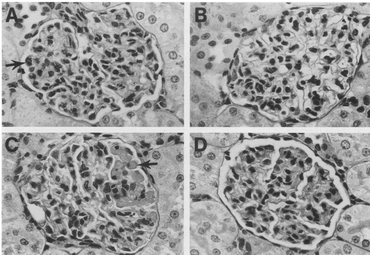
Figure 9. (A) The influx of polymorphonuclear leukocytes (arrow) in the NRS/anti-GBM Ab group (group I) was reduced in the anti-MIP-2/anti-GBM Ab group in B (group II). In C (group III), periodic acid-Schiff–positive material corresponding to fibrin-containing deposits (arrow) were also reduced after anti-MIP-2 Ab treatment shown in D (group IV). Periodic acid-Schiff stain; original magnification of 400.
