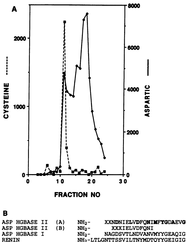
Figure 2. Vacuolar protease isolation and analysis. (A) Activity profile on hydroxylapatite HPLC chromatography. Vacuole extract was passed over DEAE-Sepharose and eluted with a NaCl gradient. The major peaks of aspartic and cysteine protease activity were pooled and fractionated on Biogel HPHT hydroxylapatite HPLC chromatography. Fractions were assayed for cysteine and aspartic protease activity. Activity measured in counts per minute product per hour. (B) Sequence analysis of aspartic hemoglobinase II. Purified enzyme was analyzed by SDS-PAGE, transferred to PVDF membrane, and subjected to NH 2 -terminal sequencing. Aligned are the two NH 2 termini obtained, along with aspartic hemoglobinase I and human renin (6). Residues identical in the two Plasmodium protease sequences are emboldened. AH, aspartic hemoglobinase.
