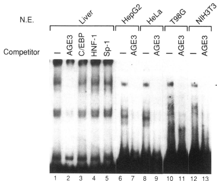
Figure 5. Identification of a ubiquitous nuclear factor (AGF3) that interacts with AGE3 (−6 to +22). (A) Electrophoretic mobility shift and competition analyses of complexes formed by factors in liver and cultured cell nuclear extracts with AGE3. Nuclear extracts from mouse liver (lanes 1–5, 10 \mu g), HepG2 (lanes 6 and 7, 10 \mu g), HeLa (lanes 8 and 9, 10 \mu g), T98G (lanes 10 and 11, 10 \mu g), and NIH3T3 cells (lanes 12 and 13, 10 \mu g) were incubated with 0.2 ng of ^{32} P-labeled AGE3. In competition assay, 100-fold molar excess of unlabeled AGE3 or double-stranded oligonucleotides (C/EBP, HNF-1, and Sp-1) was added to the reaction mixture. Arrow points to specific DNA–nuclear factor complexes. (B) DNase I footprint analysis of AGE3 with increasing amounts of liver nuclear extracts. A 160-bp HaeIII–HinfI fragment containing angiotensinogen promoter sequences from positions −138 to +22 was ^{32} P-labeled on the noncoding strand at the HinfI site. The DNA probe was incubated with mouse liver nuclear extracts (lane 3, 5 \mu g; lane 4, 10 \mu g; lane 5, 20 \mu g; lane 6, 40 \mu g) and then subjected to DNase I digestion. The hatched box to the right represents the protected region (−1 to +14) within AGE3. Nucleotide sequence of this protected region is shown, and other footprint sequences are denoted by the open boxes. The TATA box is indicated on the left. Maxam–Gilbert sequencing reactions (lane 1, G + A) of the same probe were used as markers for nucleotide positions.
