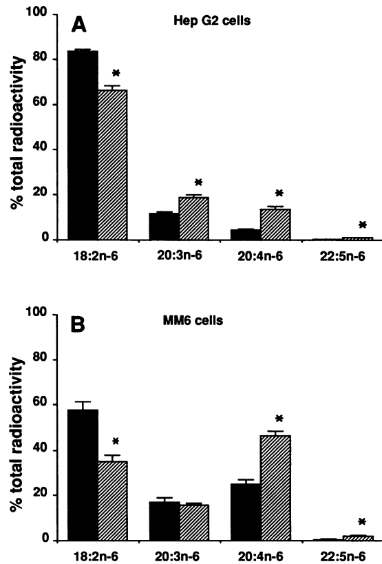
Figure 2. Effect of LOV on the desaturation of [ ^{14}\text{C} ]LA. Freshly passaged (A) Hep G2 cells and (B) MM6 cells were incubated with 10 \mu\text{M} LOV (hatched bars) or DMSO ( \leq 0.1\% , solid bars) for 72 h and with [ ^{14}\text{C} ]LA ( 0.3 \mu\text{Ci} , 5 \mu\text{M} ) for the last 18 h. Total lipids were extracted and the distribution of label in fatty acid fractions containing two, three, four, or five double bonds was determined by argentation chromatography as described in Methods. The 20:3n-6 and 20:4n-6 fractions also include the minor 18:3n-6 and 22:4n-6 fatty acids, respectively. Bars represent means \pm 1 SEM of duplicate determinations from 15 (Hep G2) and 8 (MM6) experiments. *Value is significantly different from DMSO-treated control by means of paired t test, P \leq 0.01 .
