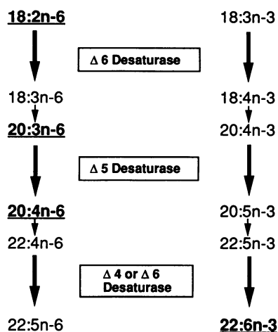
Figure 1. A schematic representation of desaturation and elongation of LA (18:2n-6) and LA (18:3n-3). Highlighted fatty acids represent major species found in animal tissues.
