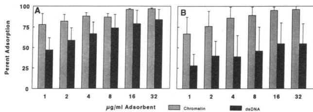
Figure 7. Absorption of (\text{H3-H4})_2 -DNA reactivity by liquid phase H1-stripped chromatin and dsDNA. Immunoabsorbent at the indicated concentrations was added to sera, incubated for 2 h at room temperature, and then ELISA performed as usual. The averages and SD for six MRL- lpr (A) and six BXSB (B) mice are displayed. As a measure of nonspecific absorption, at 4 \mu\text{g/ml} of chromatin the anti-TNP reactivity in control mice was decreased 14\% \pm 13\% .
