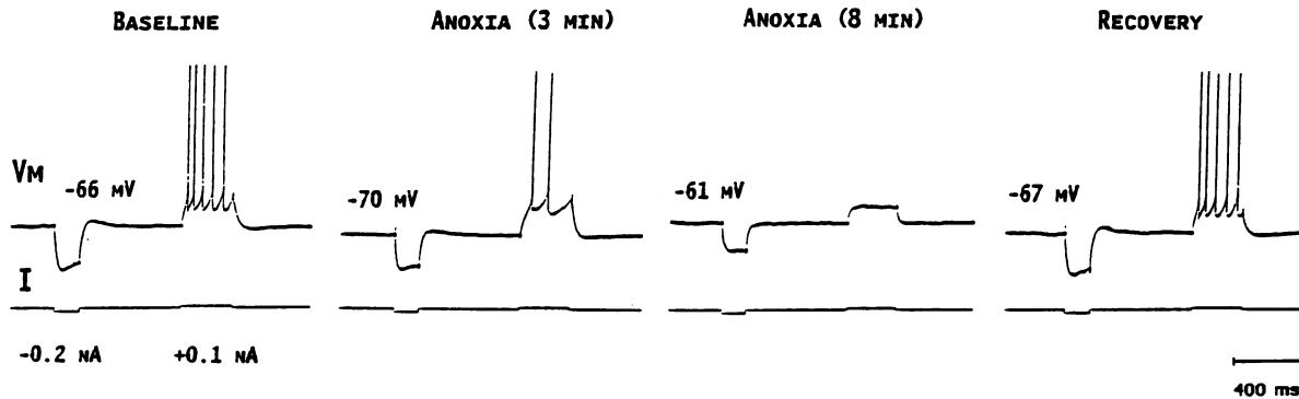
Figure 1. Electrophysiological responses of human neocortical neurons to anoxia. Intracellular recordings of a temporal cortical neuron were carried out in brain slices as previously described (12). Four short epochs extracted from continuous intracellular recordings, monitoring Vm, Rn, and neuronal activity during baseline, anoxia (3 and 8 min), and recovery. Note that (a) excitability was reduced during anoxia as action potentials ceased for the same current injection; (b) Rn decreased during anoxia; and (c) the human neocortical neuron hyperpolarized before it depolarized during the course of anoxia. After O 2 was reinstituted, Vm, Rn, and rheobase returned to the baseline level.
