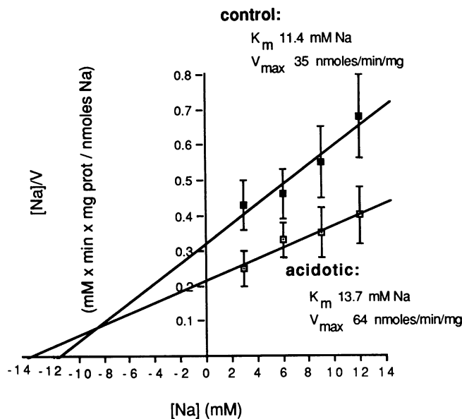
Figure 8. Kinetics of HCO 3 - -dependent Na + influx into BLM vesicles. Basolateral membrane vesicles from acidotic and control tubular suspensions were preequilibrated for 120 min at 20°C in a medium consisting of 67 mM TMA gluconate, 149 mM potassium gluconate, 52 mM Mes, 42 mM Hepes, 21 mM TMA hydroxide, pH 6.0 and gassed with 20% CO 2 . The 4-s uptake of 22 Na + into vesicles was assayed in the presence of a medium consisting of 67 mM TMA gluconate, 35 mM potassium gluconate, 114 mM potassium bicarbonate, 31 mM mannitol, 10 mM Mes, 42 mM Hepes, 31 mM TMA hydroxide pH 7.5. The Na + concentration was varied by replacing TMA gluconate with sodium gluconate in the uptake medium. Valinomycin was added at the start of preequilibration period. Values shown for uptake represent mean±SE for experiments performed in quadruplicate on four different membrane preparations.
