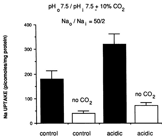
Figure 7. Effect of in vitro acidosis on \text{Na}^+:\text{CO}_3^-:\text{HCO}_3^- cotransport measured in absence of pH gradient. Basolateral membrane vesicles isolated from acidotic and control tubular suspensions were preequilibrated for 120 min at 20°C in a medium consisting of 52 mM TMA gluconate, 50 mM Na gluconate, 42 mM Hepes, 21 mM TMA hydroxide, pH 7.5 that either contained an additional 57 mM potassium gluconate and was gassed with 100% N 2 or contained 57 mM K-HCO 3 - and gassed with 10% CO 2 , 90% N 2 . The 10-s uptake of 2 mM 22 Na + into basolateral membrane vesicles was assayed in the presence of a medium consisting of 52 mM TMA gluconate, 48 mM TMA gluconate, 2 mM Na gluconate, 42 mM Hepes, 21 mM TMA hydroxide, pH 7.5 that either contained an additional 57 mM potassium gluconate and was gassed with 100% N 2 or contained 57 mM K-HCO 3 - and gassed with 10% CO 2 , 90% N 2 . Values shown for uptake represent mean±SE for experiments performed in quadruplicate on four different membrane preparations.
