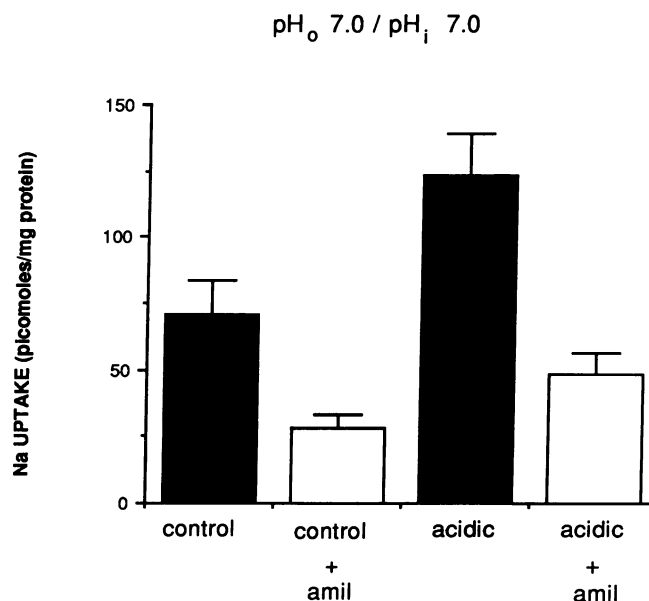
Figure 3. Effect of in vitro acidosis on \text{Na}^+/\text{H}^+ exchange measured in absence of pH gradient. Brush border membrane vesicles from acidotic and control tubular suspensions were preequilibrated for 120 min at 20^\circ\text{C} in a medium consisting of 52 mM TMA gluconate, 165 mM potassium gluconate, 39 mM mannitol, 13 mM Mes, 42 mM Hepes, 21 mM TMA hydroxide, pH 7.0. The 10-s uptake of 1 mM ^{22}\text{Na}^+ into brush border membrane vesicles was assayed in the presence of a similar medium at pH 7.0. Values shown for uptake represent mean \pm SE for experiments performed in quadruplicate on four different membrane preparations.
