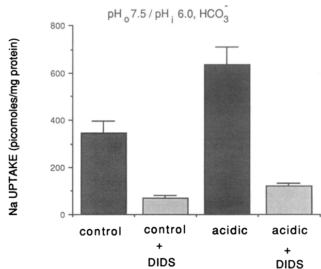
Figure 6. Effect of DIDS on \text{HCO}_3^- -dependent \text{Na}^+ influx in BLM vesicles. The 10-s uptake of 1 mM ^{22}\text{Na}^+ into the basolateral membrane vesicles preequilibrated in pH 6.0 medium was assayed in the presence of 57 mM \text{HCO}_3^- , 20% \text{CO}_2 at pH 7.5 as described in Fig. 5. DIDS (0.5 mM) was added as the disodium salt to the external solution. Valinomycin was added at the start of the preequilibration period. Values shown for uptake represent mean \pm SE for experiments performed in quadruplicate on four different membrane preparations.
