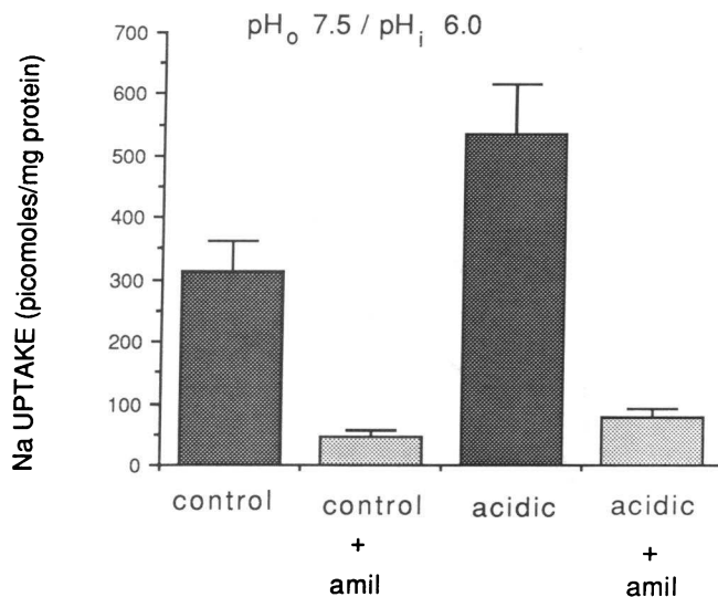
Figure 2. Effect of amiloride on pH-dependent \text{Na}^+ influx. The 10-s uptake of ^{22}\text{Na}^+ into brush border membrane vesicles preequilibrated in pH 6.0 medium was assayed in the presence of pH 7.5 medium as described in Fig. 1. Amiloride (1 mM) was added as the hydrochloride salt to the external solution. Valinomycin was added at the start of preequilibration period. Values shown for uptake represent mean \pm SE for experiments performed in quadruplicate on four different membrane preparations.
