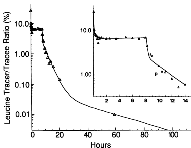
Figure 2. Plasma leucine tracer/tracee ratio after a primed constant infusion of [1- 13 C]leucine in subject 1. A triexponential function was computer fitted (line) to observed plasma leucine tracer/tracee ratios (symbols) as described previously (19). This function was subsequently used as a forcing function to describe the input of the tracer for the modeling process.
