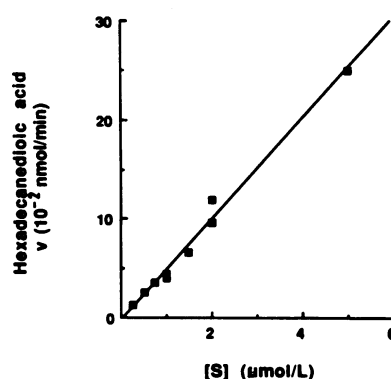
Figure 3. The omega-oxidation of laurate and palmitate. The omega-oxidation of varying concentrations of [1-^{14}\text{C}] laurate (A) and [9,10(n)-^3\text{H}] palmitate (B) was assessed by measuring the formation of dodecanedioic or hexadecanedioic acid using 2 mg of postmitochondrial supernatant from rats treated with acetylsalicylic acid for 2 wk. The lines in A and B are described by the equations y = 0.144 + 1.04x , r^2 = 0.973 and y = 0.259 + 5.095x , r^2 = 0.987 .
