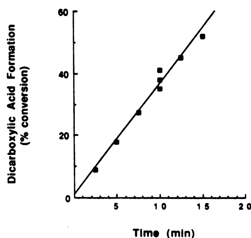
Figure 2. Laurate omega-oxidation as a function of protein concentration and time. (A) The omega-oxidation of 2 \mu\text{M} [1-^{14}\text{C}] -laurate was assessed by determining the formation of dodecanedioic acid formation at 37^\circ\text{C} for 10 min in a reaction using varying amounts of postmitochondrial supernatant from rats treated with acetylsalicylic acid for 2 wk. (B) The omega-oxidation of 2 \mu\text{M} [1-^{14}\text{C}] -laurate was assessed at varying times by measuring the formation of dodecanedioic acid in a reaction mixture containing 2 mg of postmitochondrial supernatant as described above. The lines in A and B are described by the equations y = 1.207 + 16.864x , r^2 = 0.945 and y = 0.971 + 3.549x , r^2 = 0.978 , respectively.
