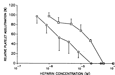
Figure 3. Heparin inhibition of bovine von Willebrand factor. Formaldehyde fixed washed platelets resuspended in TBS with 1% BSA were directly agglutinated with purified bovine vWF (20 \mu\text{g}/\text{ml} ) after preincubation with
