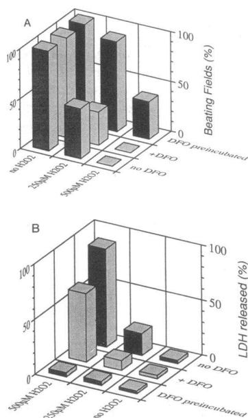
Figure 2. Effect of DFO on H_2O_2 -induced loss of cellular LDH and contractility of cardiomyocytes. Varying concentrations of H_2O_2 were incubated for 80 min with monolayered beating cardiomyocytes. The effect of 0.1 mM DFO, either preincubated with the cells for 2 h or added together with H_2O_2 , was studied by determining the residual fraction of "beating microscopic fields" (A) and LDH released extracellularly (B).
