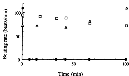
Figure 1. Effect of nitroxides on H 2 O 2 -induced loss of cell contractility. The beating rate of isolated rat heart cells after the incubation with 250 \mu\text{M} H 2 O 2 in the absence (circles) and the presence of (triangles) of 0.5 mM compound II or (squares) of 0.5 mM Tempo. The plated cells were kept at 37°C in Ham F-10 culture medium under atmosphere of 5% CO 2 and 95% air.
