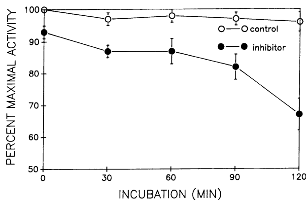
Figure 4. Inactivation of purified beef brain \alpha -KDHC by \Delta 2,3 VPE. The complex (0.1 mg/ml) was incubated at 25°C in 50 mM MOPS, 2 mM \text{MgCl}_2 , 0.5 mM \text{CaCl}_2 , 2.6 mM cysteine, 0.1 mM TPP, pH 7.6, either in the presence of 2 mM \Delta 2,3 VPE (inhibitor) or not (control). Aliquots taken at intervals were assayed as described in the text. Each data point represents the mean of duplicate determinations from three experiments, with error bars indicating 1 SD. The ordinate represents percentage of initial rate activity of an untreated sample. At 120 min, activity in the preincubated samples was significantly lower than control ( P < 0.005 ).
