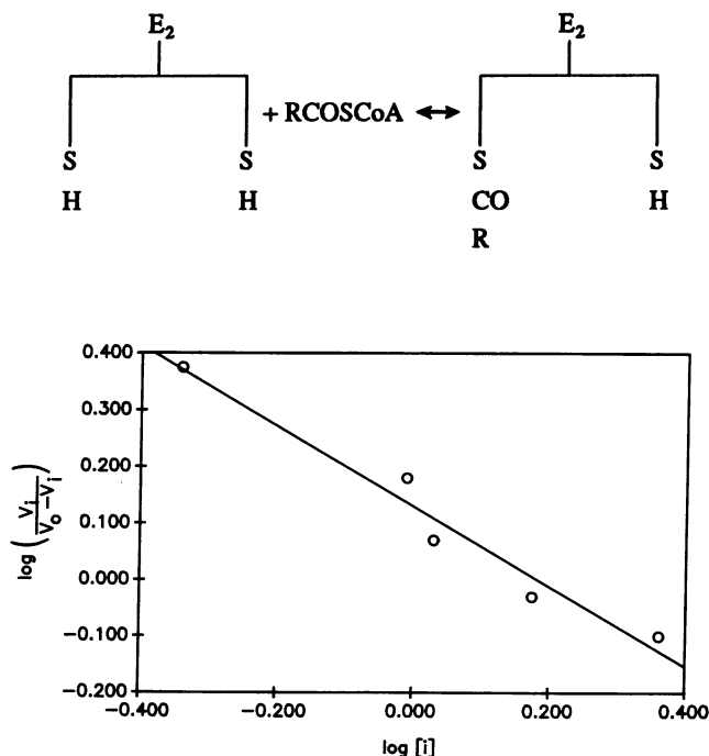
Figure 9. Inhibition of purified beef brain \alpha -KDHC by \delta 2,3 VPE-CoA. Results are presented as a Hill plot. V_i is the initial rate of reaction in the presence of inhibitor and V_0 the rate under the same conditions without inhibitor. CoA concentration was 1.3 \mu\text{M} (=K_m) . Other substrates were as described in the text.
