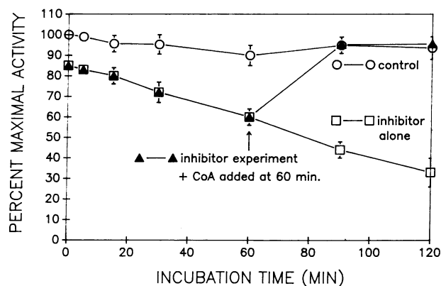
Figure 5. Inactivation of purified beef brain \alpha -KDHC by \Delta 2,3 VPE-CoA. The complex (0.1 mg/ml) was incubated at 25°C in 50 mM MOPS, 2 mM \text{MgCl}_2 , 0.5 mM \text{CaCl}_2 , 0.1 mM cysteine, 0.1 mM TPP, pH 7.6, either in the presence of 1 mM \Delta 2,3 VPE-CoA (inhibitor) and 1 mM NADH or in 1 mM NADH only (control). Aliquots were taken at intervals and assayed as described in the text. Each data point represents the mean of duplicate determinations from three experiments, with error bars indicating 1 SD. The ordinate represents percentage of initial rate activity of an untreated sample. Activity at 90 and 120 min was significantly lower in the preincubated samples ( P < 0.01 90 min, P < 0.001 120 min). No significant difference in activity from control if 0.5 mM CoA was added to aliquots at 60 min and assayed at 90 and 120 min. Incubation with VPA-CoA gave similar results.
