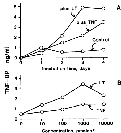
Figure 9. Production of TNF-BP from HL-60 cells. Cells ( 10^6 /ml at the start point) were incubated for 4 d (A) with 1,000 pmol/liter lymphotoxin (LT), 1,000 pmol/liter TNF or without added cytokine. Incubations were also performed in the presence of various concentrations of lymphotoxin and TNF (B). TNF-BP of cell supernatants was determined with an ELISA.
