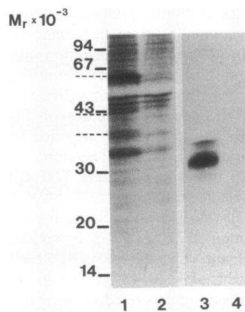
Figure 8. Immunoprecipitation with anti-TNF-BP of biosynthetically labeled HeLa cells. The cells were labeled with ^{35}\text{S} -cysteine for 30 min. The cell extract was immunoprecipitated with anti-TNF-BP (lane 1) or preimmune serum (lane 2). In another experiment cells were labeled with ^{35}\text{S} -cysteine for 30 min followed by chase of the label for 60 min in the presence of 10 ng/ml PMA after which the cell supernatant was immunoprecipitated with anti-TNF-BP (lane 3) or preimmune serum (lane 4). Molecular weight standards are indicated to the left. Arrow indicates the position of TNF-BP. Broken lines indicate the position of intracellular components precipitated with anti-TNF-BP.
