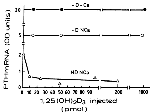
Figure 3. 1,25(\text{OH})_2\text{D}_3 dose-response effect on parathyroid gland PTH mRNA 24 h after intraperitoneal injections, to rats on control diets (NDNCa) (from reference 8); vitamin D-deficient, normal calcium ( -D\text{-NCa} ) and calcium-deficient ( -D\text{-Ca} ). The results represent the mean for four rats.
