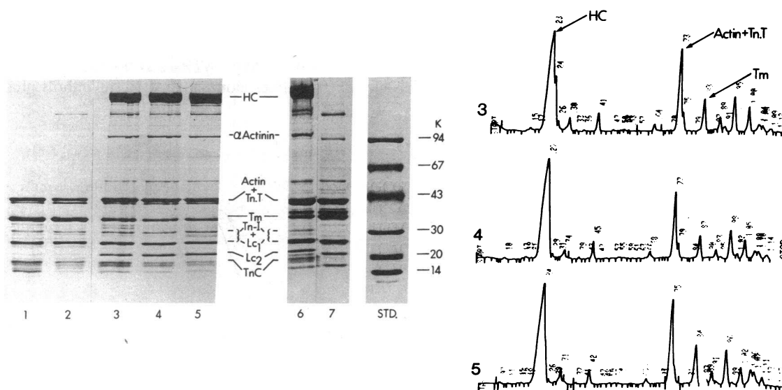
Figure 1. SDS gradient slab gel (5.0–16.5%) and densitometric scans of cardiac myofibrils (MF) hybridized with the cold cardiac Tn.Tm complex from normal dog (D), control (C) and myopathic (M) hamsters. Lane 1, Tn.Tm (C); lane 2, Tn.Tm (M); lane 3, MF (C); lane 4, MF(M); lane 5, MF(M) plus Tn.Tm (C); lane 6, MF [M] plus Tn.Tm (D); lane 7, Tn.Tm (D) complex; and lane 8, standard molecular weight protein markers. On the right are the densitometric scans of preparations from lanes 3, 4, and 5. HC, heavy chains; LC 1 , light chain-1; LC 2 , light chain-2; Tm, tropomyosin; Tn-I, troponin-I; Tn-T, troponin T; and Tn-C = troponin-C.
