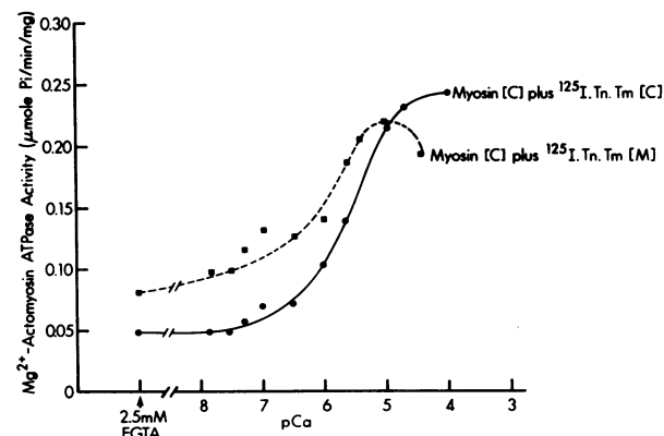
Figure 5. \text{Mg}^{2+} ATPase of reconstituted actomyosin as a function of free \text{Ca}^{2+} ion in the presence of cardiac ^{125}\text{I} -Tn.Tm complex isolated from control (C) and myopathic (M) hamsters. The number of preparations for each curve is two.
