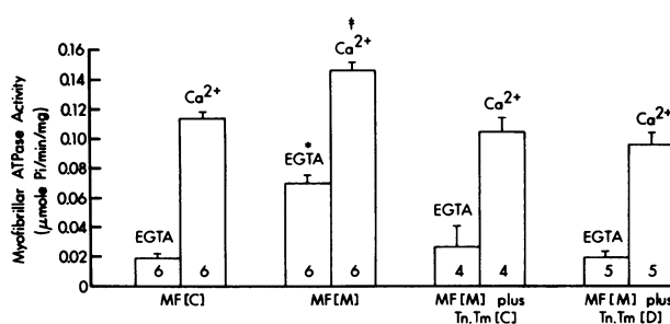
Figure 3. Cardiac myofibrillar ATPase activity plotted in the absence of \text{Ca}^{2+} ( \text{Mg}^{2+} ATPase) and in the presence of 0.1 \text{ mM Ca}^{2+} ion ( \text{Ca}^{2+} \text{Mg}^{2+} ATPase). Results are mean \pm SE. The number of experiments are indicated in each bar. * indicates P < 0.05 when comparing \text{Mg}^{2+} ATPase for MF[M] with all other groups. † indicates P < 0.05 while comparing \text{Ca}^{2+} \text{Mg}^{2+} ATPase of MF[M] against all other preparations.
