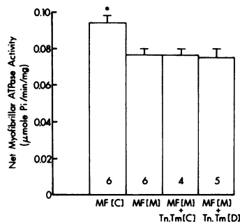
Figure 4. Net \text{Ca}^{2+} myofibrillar ATPase activity ( \text{Mg}^{2+} ATPase subtracted from total \text{Ca}^{2+} \text{Mg}^{2+} myofibrillar ATPase activity; 0.1 \text{ mM Ca}^{2+} ) of myofibrils. Designations for columns 1, 2, 3, and 4 are the same as in Fig. 3.
