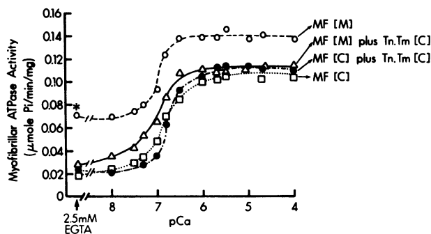
Figure 2. Cardiac \text{Ca}^{2+} \text{Mg}^{2+} activated myofibrillar ATPase vs. free calcium concentration. Myofibrils from control (MF[C]); myopathic (MF[M]); control myofibrils mixed with control troponin-tropomyosin complex (MF[C] plus Tn.Tm [C]); and myopathic myofibrils plus control Tn.Tm (MF [M] plus Tn.Tm [C]). Mean results are for four to seven different preparations; two experiments each for every preparation. * indicates P < 0.05 when \text{Mg}^{2+} ATPase for MF[M] is compared with all other myofibrillar \text{Mg}^{2+} ATPase(s).
