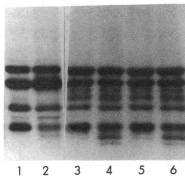
Figure 7. Autoradiographs of SDS gels of the four different myofibrillar preparations from C and M hamster hearts hybridized with ^{125}\text{I} -Tn.Tm from C and M hearts. Numbers 1–6 are the autoradiographs of lanes 1–6 in Fig. 6.
