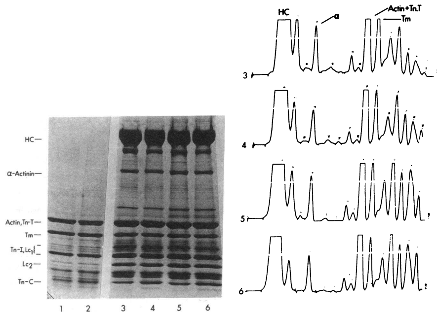
Figure 6. SDS gradient slab gel (5.0–16.5%) and densitometric scans of the cardiac myofibrils hybridized with ^{125}\text{I} -Tn.Tm in control (C) and myopathic (M) hamster hearts and vice versa. Lane 1, ^{125}\text{I} -Tn.Tm (C); lane 2, ^{125}\text{I} -Tn.Tm(M); lane 3, MF (C) plus ^{125}\text{I} -Tn.Tm (C); lane 4, MF (C) plus ^{125}\text{I} -Tn.Tm(M); lane 5, MF (M) plus ^{125}\text{I} -Tn.Tm (C); and lane 6, MF(M) plus ^{125}\text{I} -Tn.Tm(M).
