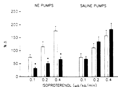
Figure 2. The effects of acute challenges to isoproterenol ( 0.1 – 0.4 \mu\text{g/kg} per min) on left ventricular dP/dt were examined before (open bars) and after (solid bars) implantation of the miniosmotic pumps. Animals with NE pumps are shown
