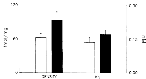
Figure 3. \beta -Adrenergic receptor density and K_d as determined by Scatchard analysis using ^{125}\text{I} -cyp are shown for animals with saline pumps (open bars) and animals with NE pumps (solid bars). \beta -Receptor density is significantly increased ( P < 0.05 ) in the animals with NE pumps as compared with animals with saline pumps. There is no difference in K_d between the two groups. * P < 0.05 .
