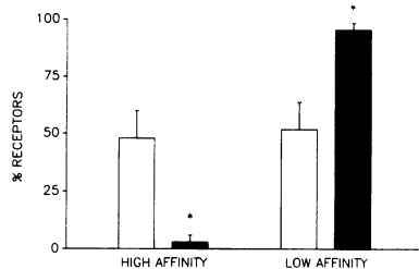
Figure 4. \beta -Adrenergic receptor competitive inhibition agonist binding with isoproterenol and ^{125} I-cyp was performed for animals with saline pumps (open bars) and animals with NE pumps (solid bars).
