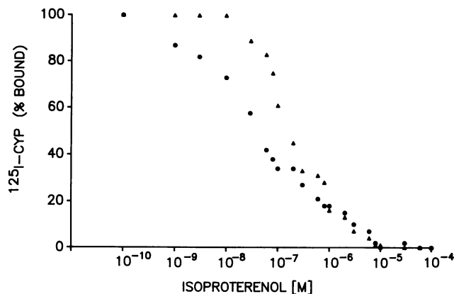
Figure 6. Isoproterenol agonist binding with the purified membrane preparation and 0.1 \text{ nM } ^{125}\text{I-cyp} with increasing concentrations of isoproterenol is shown for the left ventricle from an animal with a saline pump (circles) and an animal with a NE pump (triangles). The NE pump curve is shifted to the right, indicating a shift toward a single, low affinity site.
