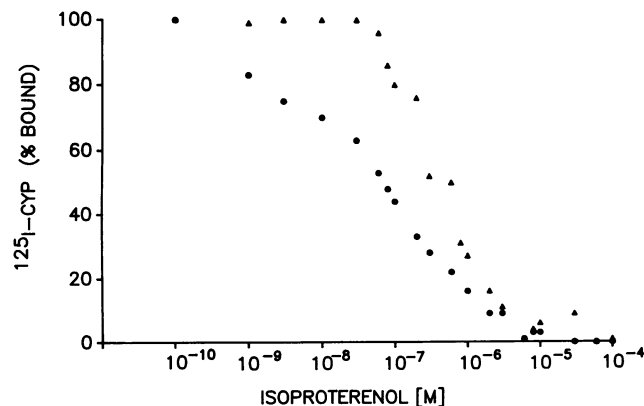
Figure 5. Isoproterenol agonist binding with the crude membrane preparation, and 0.1 \text{ nM } ^{125}\text{I-cyp} with increasing concentrations of isoproterenol is shown for the left ventricle from an animal with a saline pump (circles) and an animal with a NE pump (triangles). The NE pump curve is shifted to the right, indicating a shift toward a single, low affinity site.
