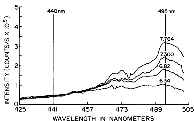
Figure 1. Excitation spectra of intracellular BCECF in OMCDi. OMCDi were loaded with 2 \mu\text{M} BCECF-AM for 10 min at 37^\circ\text{C} . Fluorescent emission intensity between 520–560 nm was recorded. The excitation wavelengths were scanned from 425–505 nm. Spectra were obtained while intracellular pH was clamped using four different HEPES buffered, high \text{K}^+ /nigericin baths set at pH 6.34, 6.82, 7.30, and 7.76 ( 37^\circ\text{C} ). It can be seen that emission intensity using 440 nm excitation was pH insensitive, while emission using 495 nm excitation was highly dependent on pH.
