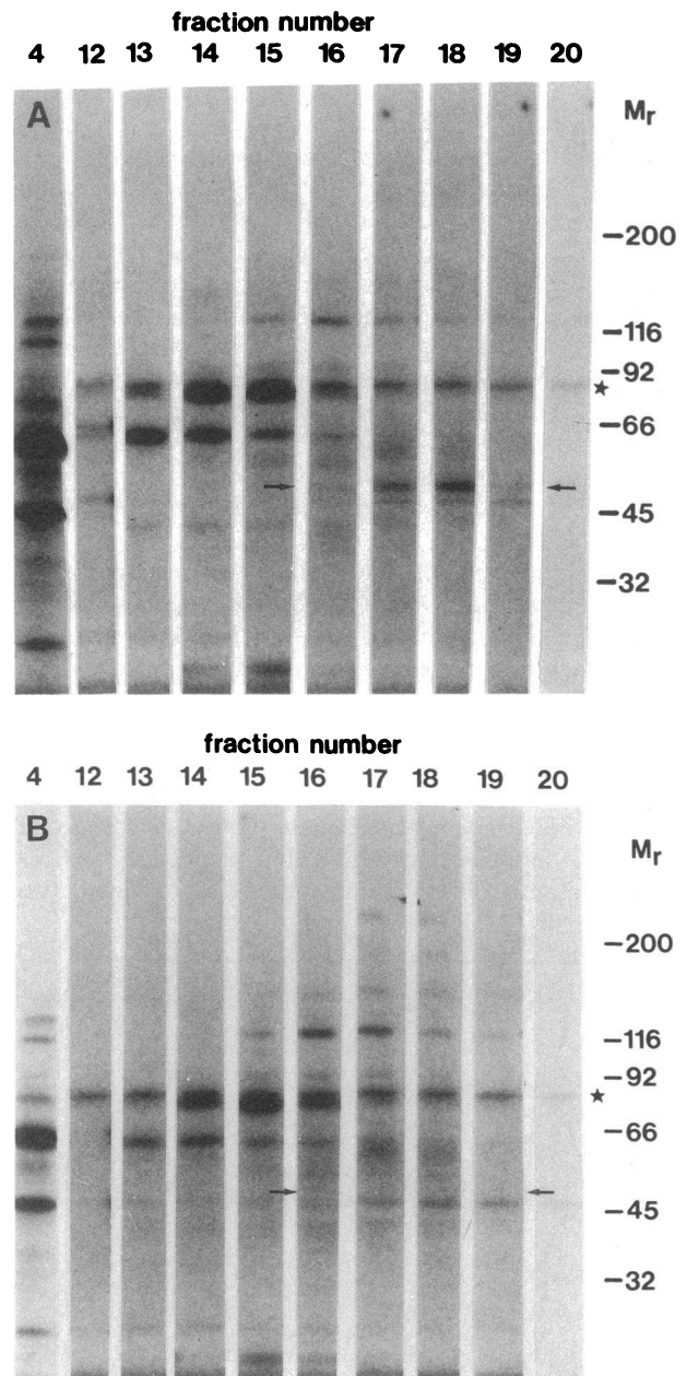
Figure 3. (A) Autoradiograph of SDS-PAGE gel of CM-Sepharose fractions. Samples of 50\ \mu\text{l} from the CM Sepharose fractionation (Fig. 1) were phosphorylated in vitro with purified protein kinase C as described in Methods. SDS-PAGE was run in a 5–15% polyacrylamide gel. (B) Autoradiograph of SDS-PAGE gel of CM-Sepharose fractionation of the soluble fraction from autosomal CGD neutrophils. Soluble fraction of autosomal CGD neutrophils ( 120 \times 10^6 cell equivalents) was separated on CM Sepharose in parallel to a control experiment as described in Fig. 1. A gradient of 0–200 mM NaCl (0–12.5 ml) was applied, and fractions of 2.2 ml were collected. 100\ \mu\text{l} of the fractions was phosphorylated in vitro with protein kinase C as described in Methods. SDS-PAGE was run in a 5–15% polyacrylamide gel, followed by autoradiography of the gel. The numbers of the fractions correspond to the control experiment in Fig. 1 and Fig. 3 A. The arrows show the level of M_r 47,000. The asterisks indicate protein kinase C autophosphorylation.
