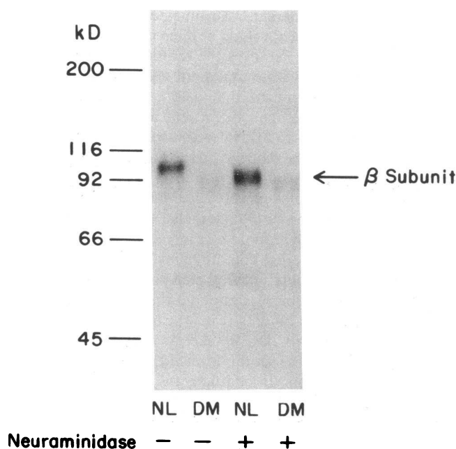
Figure 10. Effect of neuraminidase on WGA-purified insulin receptor \beta subunit of endothelial cells from diabetic and nondiabetic BB rats. The details of the study is described in Methods. Receptors from nondiabetic rats with (lane 1) and without (lane 3) neuraminidase treatment. Lanes 2 and 4 represented receptors from diabetic rats.
