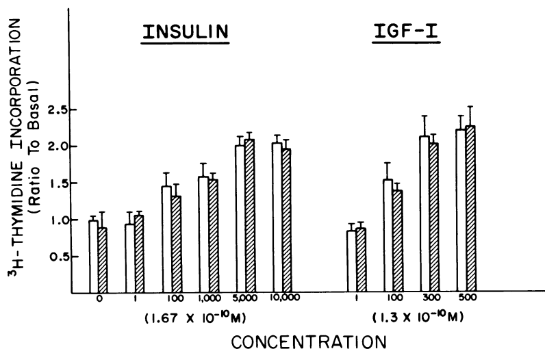
Figure 3. Dose response of insulin- and IGF-I-stimulated DNA synthesis as measured by [ ^3 H]thymidine incorporation in capillary endothelial cells from (■) diabetic and (▨) nondiabetic BB rats. [ ^3 H]Thymidine incorporation was performed as described in Methods. Data shown here are mean and SE from three separate experiments. The difference between diabetic and nondiabetic is not significant.
