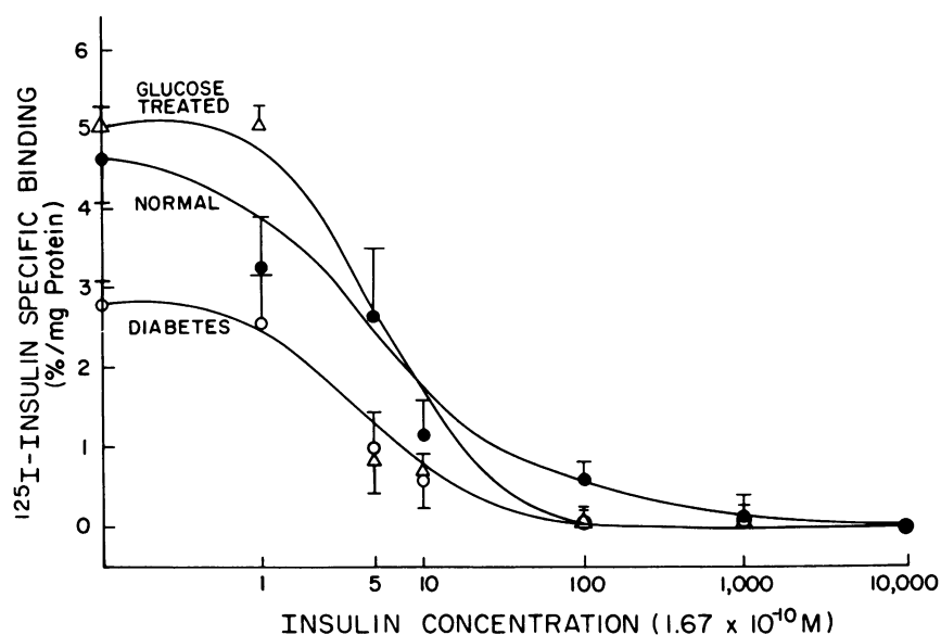
Figure 4. Competitive inhibition curves of insulin binding to intact capillary endothelial cells of (○) diabetic and (●) nondiabetic BB rats and (Δ) cells from nondiabetic rats and treated with high glucose (400 mg/dl) for 1–10 mo in culture. Insulin binding to endothelial cells was performed as described in Methods. The specific binding was calculated by subtracting the amount of radioactivity bound in the presence of 1.6 \times 10^{-6} M ( 10 \mu\text{g/ml} ) of unlabeled porcine insulin from the total radioactivity bound to cells. Each point represents mean and SE from five separate experiments using endothelial cells from five different groups of diabetic and nondiabetic BB rats.
