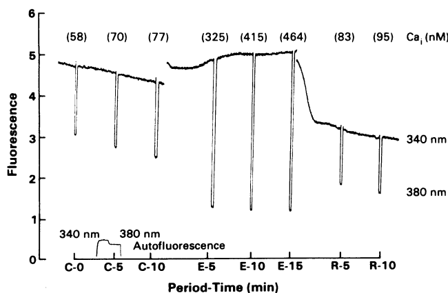
Figure 2. Representative experiment of the effect of cyanide and 2-deoxy-D-glucose on Ca_i . The format is the same as in Fig. 1. On the abscissa C, E, and R represent control, experimental, and recovery periods, respectively. Fluorescent ratios were measured at 5-min intervals. During the 15-min experimental period the superfusate contained cyanide and 2-deoxy-D-glucose without glucose. Immediately after the E-15 measurement, the superfusate is changed to the control solution for the 10-min recovery period. Ca_i rises during the experimental period and recovers rapidly with removal of cyanide and 2-deoxy-D-glucose.
