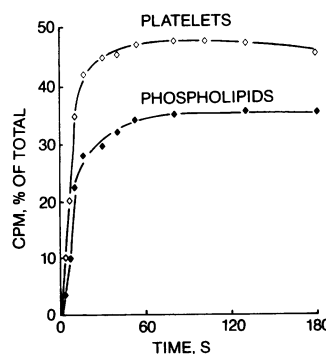
Figure 1. Rate of incorporation of [ ^3\text{H} ]palmitic acid (170 nM) into rabbit platelets and into phospholipids. Platelets ( 500,000/\mu\text{l} ) in a modified Tyrode solution (no \text{Ca}^{2+} , no albumin) were incubated with [ ^3\text{H} ]palmitic acid for the times indicated. Samples were centrifuged and the supernatants counted to determine (by difference) the amount of radioactivity associated with the platelet pellet. Platelets were
