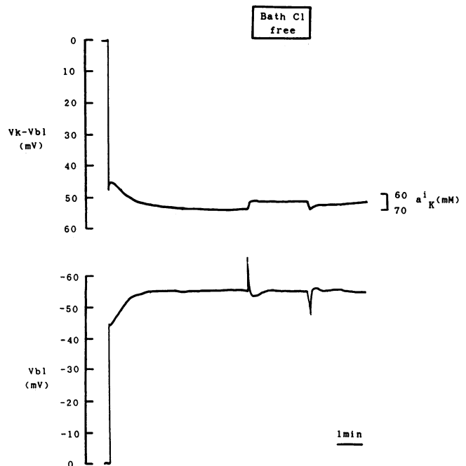
Figure 5. Effect of eliminating bath Cl^- on a_K^i . Bath Cl^- was replaced with gluconate.
