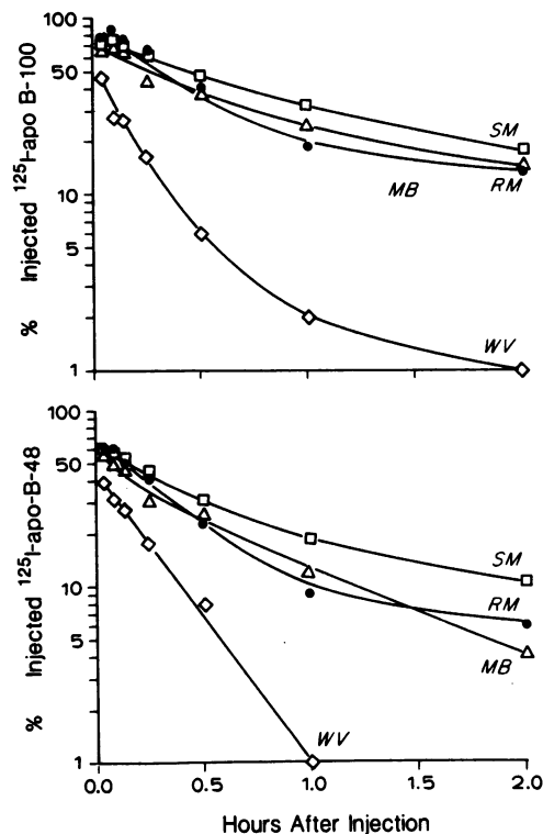
Figure 3. Removal of ^{125}\text{I} -apo B-100 and ^{125}\text{I} -apo B-48 from TG-rich lipoproteins of blood plasma of the four normolipidemic subjects during the first 2 h after injection. Data are the same as those shown in Fig. 2 and are depicted on an expanded time scale. An appreciable fraction of ^{125}\text{I} was removed from apo B-100 and apo B-48 within 2 min, in some cases followed by plateau before further removal occurred (see text).
